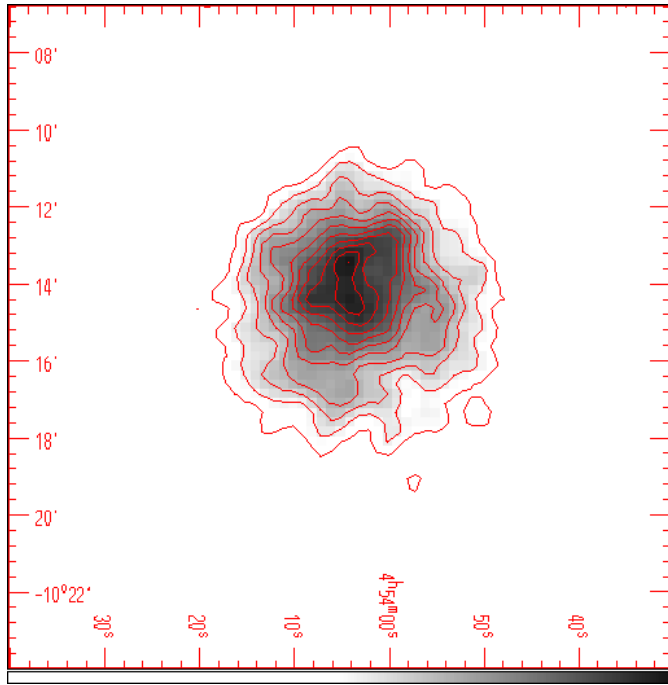
Fig. 5. The smoothed ASCA GIS image of A521; the GIS2 and GIS3 images are combined. The contours are 0.275 – 1.25 counts/s/arcmin 2 and the difference between adjacent contours is 0.0975. The image is smoothed by a gaussian filter with \sigma = 15'' .
