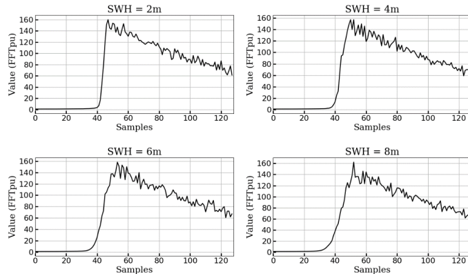
Figure 1: Example of waveforms simulated for four SWH steps (2m, 4m, 6m and 8m), after application of speckle noise and thermal noise. The Y axis represents the amplitude in FFT power units.
