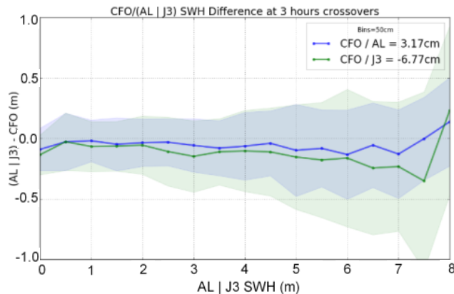
Figure 14: Bias between SWIM SWH and two altimeter missions (SARAL/AltiKa in blue, Jason-3 in green) for SWIM cycle 21 to 28. Each dot of the solid line is the mean computed per box of 50cm of SWH and the envelope represents the associated standard deviation
