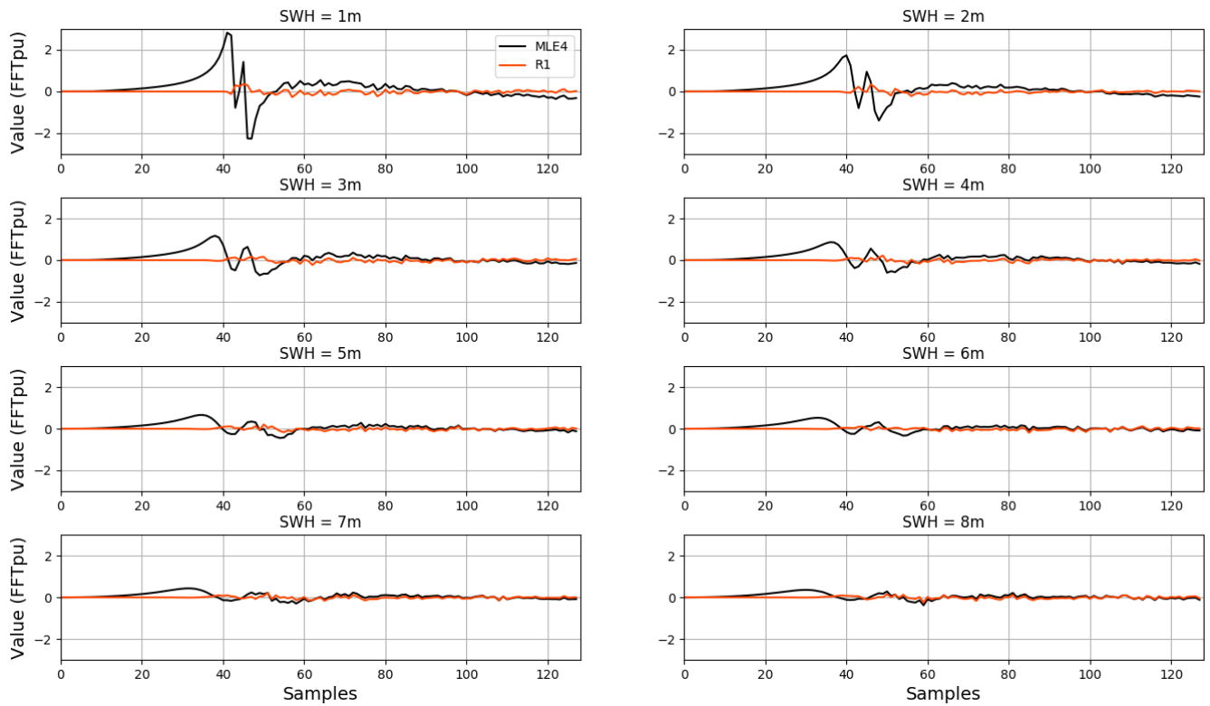
Figure 2 : Differences between fitted echoes and the reference waveforms over all samples for a retracking processing with MLE4 algorithm with modeled PTR convolution (black curve) and R1 retracking with real PTR convolution (red curve). The Y axis represents the amplitude in FFT power units.
