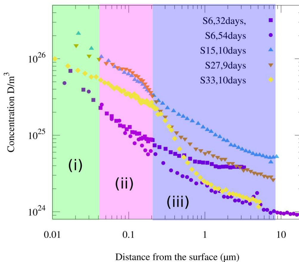
Fig. 8. SIMS depth profiling of deuterium content of damaged Eurofer samples. Irradiation doses: S6 – 0 dpa, S15 – 0.01 dpa, S27 – 0.1 dpa, and S33 – 1 dpa. Time delay between exposure to deuterium plasma and the SIMS is given in days.
