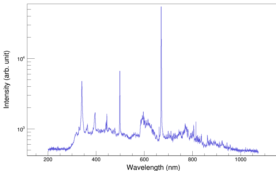
Fig. 6. An example spectrum taken during the exposure of a sample using recirculating deuterium. The D_{\beta} and D_{\alpha} lines can be seen at 486 nm and 656 nm respectively, along with the Fulcher band between 560 nm and 640 nm. This spectrum indicates no significant buildup of impurities caused by re-circulation of the deuterium through the plasma chamber, suggesting deuterium results can be compared with those from other systems which typically have a ‘once through’ setup and exhaust the deuterium from the exposure chamber.
