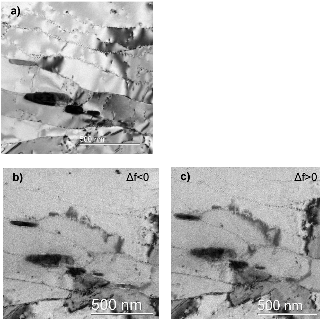
Fig. 9. TEM in-situ pictures of Eurofer sample irradiated to 1 dpa. Initial microstructure (a), microstructure at 625°C indicating cavities formed along grain boundaries and precipitates by change of contrast (b,c).
