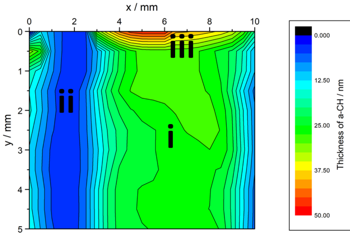
Fig. 3. An ellipsometry survey of an a-C:H foil exposed to 100 eV deuterium ions for 20 minutes. Region (i) shows approximately uniform erosion by the beam in the central area where the sample is located. Region (ii) shows where the left-hand retaining clip held the foil in place, and similarly the imprint of the right-hand clip can be seen to the right of the figure. Region (iii) shows where the top of the foil was shielded from the ion flux by a molybdenum foil shield and so the amount of erosion reduces sharply.
