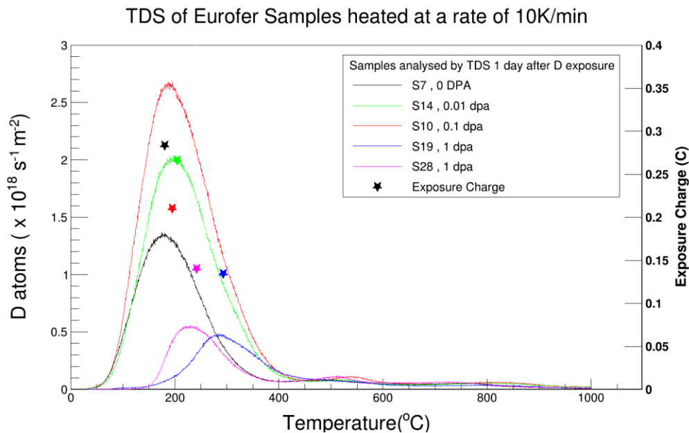
Fig. 7. TDS spectra of deuterium and exposure charge in Eurofer samples with damage levels between 0 and 1 dpa. Time period between exposure to deuterium plasma and the TDS is 1 day for all samples. The lower limit of the charge incident on the sample is indicated. It can be seen that the retention is more strongly affected by the damage level than the ion fluence.
