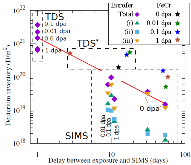
Fig. 12. The total retention in Eurofer and Fe-Cr samples as a function of delay between exposure and analysis.
