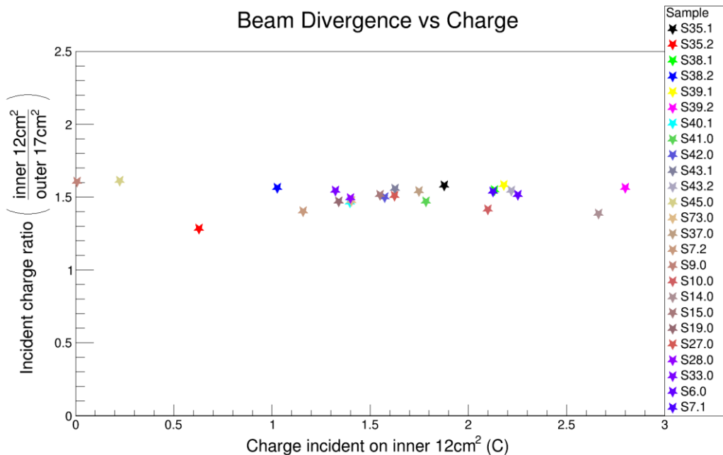
Fig.5. The ratio of ions incident on the inner and outer plates, providing an indication of beam divergence. The ratio of the areas of these plates is 0.7.
