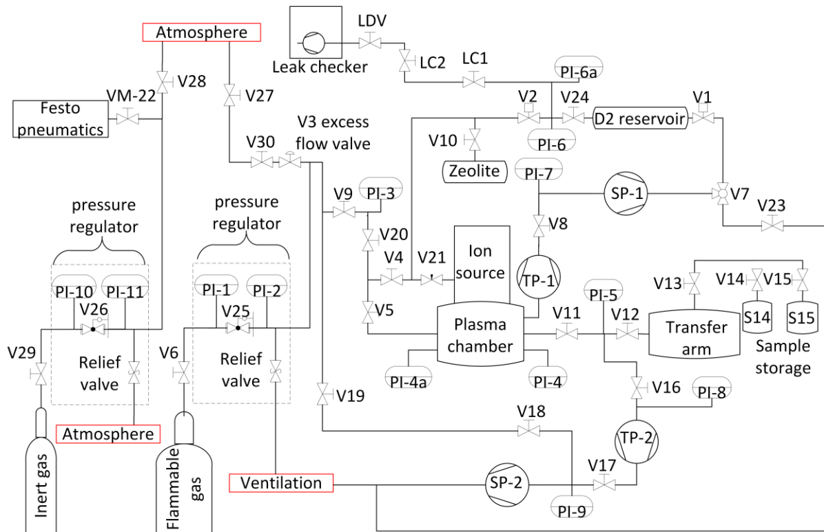
Fig. 2. Piping and Instrumentation Diagram (P&ID) of deuterium exposure system.
