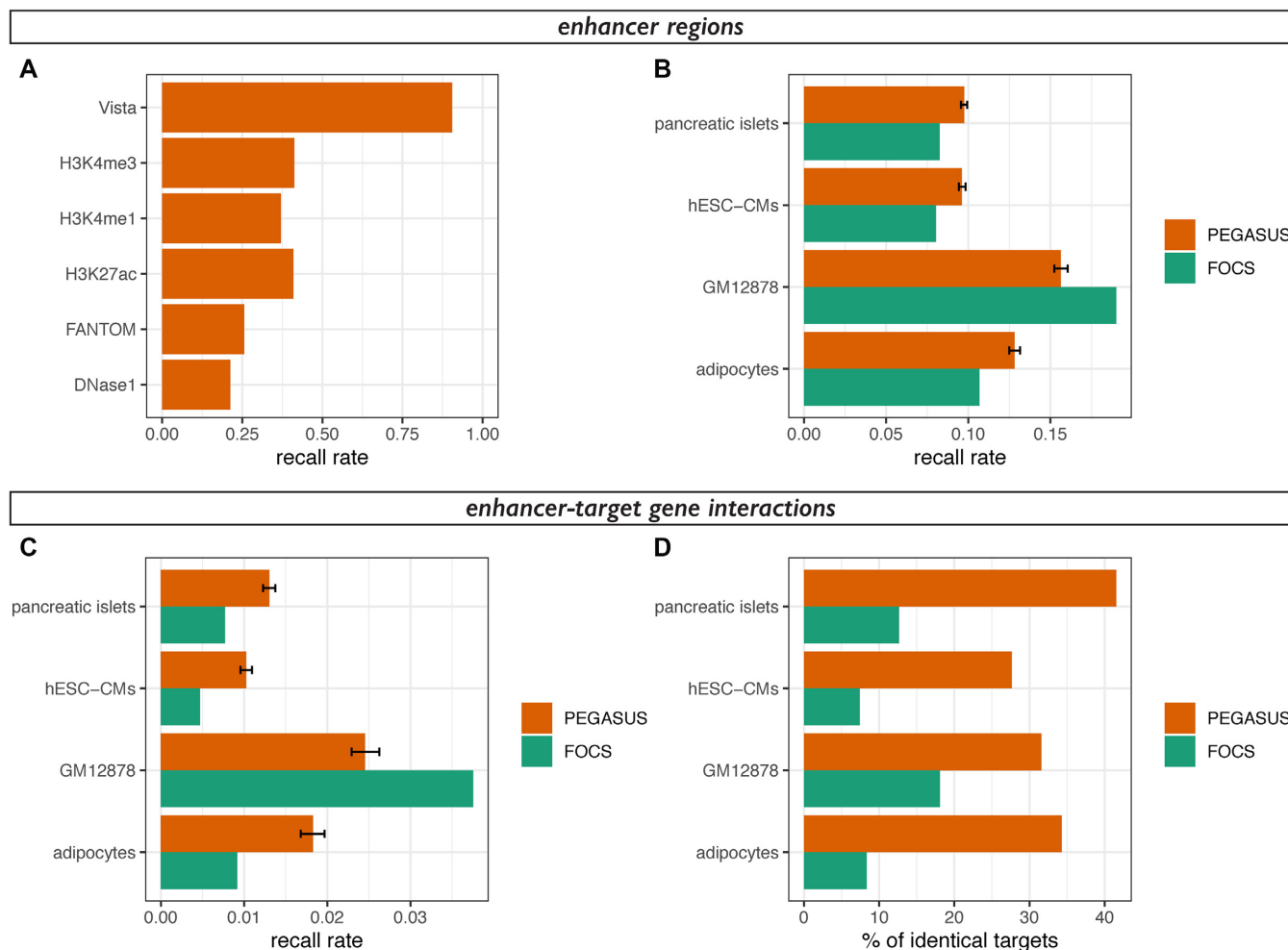
Figure 3. Overlap between enhancer-target gene prediction methods. (A) Recall rates (1 – false negative rate) for predicted enhancer regions in the human genome. Predicted enhancer regions are the same as in Figure 2. (B) Recall rates for enhancer regions of cHi-C data in adipocytes (20), GM12878 cells (21), embryonic stem cell-derived cardiomyocytes (22) and pancreatic islets (23). Recall rates were computed from PEGASUS enhancers (orange) or FOCS enhancers (25) using the same number of interactions in both sets. Mean recall rates and 2.5–97.5 percentiles (error bar) of 1000 random samplings were plotted for PEGASUS. For each dataset, recall rates for FOCS predictions are significantly different from recall rates for PEGASUS predictions (all P -values < 10^{-35} ). (C) Recall rates for enhancer-target gene interactions of cHi-C data in the same cell types as (B). The colour code is identical as (B) and the same number of interactions were used in both sets. Mean recall rates and 2.5–97.5 percentiles (error bar) of 1000 random samplings were plotted for PEGASUS. For each dataset, recall rates for FOCS predictions are significantly different from recall rates for PEGASUS predictions (all P -values < 10^{-36} ). (D) Percentage of agreement between in-silico predictions methods (PEGASUS or FOCS) and in-vitro cHi-C interactions, computed as the percentage of one to one overlapping enhancers predicted to target the same gene (see Materials and Methods for more details). We analysed 1755 interactions for pancreatic islets, 1751 interactions for hESC-CMs, 326 interactions for GM12878 cells and 767 interactions for adipocytes.
