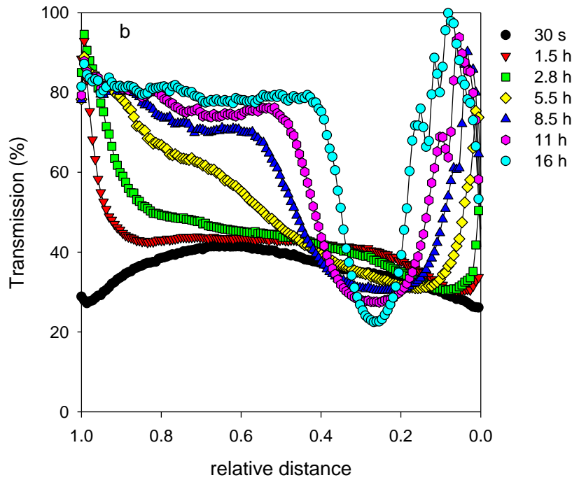
Fig. 1 Transmission profiles of emulsions without (a) and with 1 g/L chitosan (b) at different times during centrifugation at 30G.
