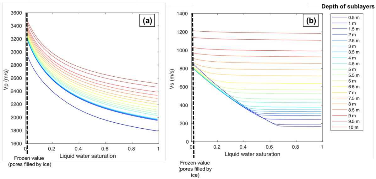
885 Figure 11: (a) Evolution of P-wave velocity V_p with respect to the ratio between water and ice filling the pores, resulting from the Biot-Gassmann type three-phase poroelastic model, applied to the Laurichard rock glacier (for C00 seismometer). The different curves correspond to the different sublayers, whose depth is indicated in the right panel. The V_p values used to model the winter state are those for liquid water saturation tending towards zero. (b) Same results for S-wave velocity V_s .
