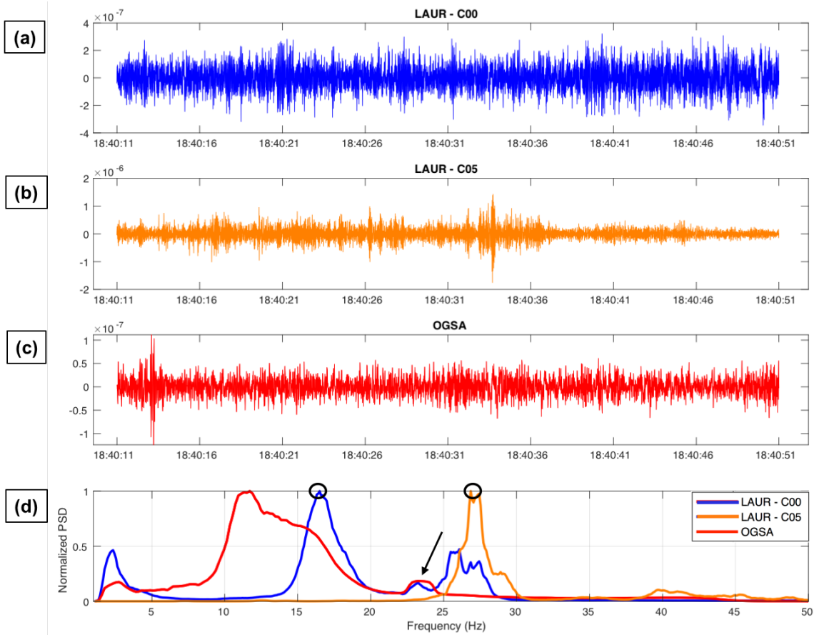
830 Figure 2: Seismic recordings of ambient noise (vertical ground velocity in m/s, after >1 Hz filtering and instrumental deconvolution) recorded by sensors C00 (a) and C05 (b) in Laurichard rock glacier, and by OGSA station at Lautaret pass (c), the 5 th April 2019 at 6 PM. (d) The normalized PSD of the respective signals. Black circles highlight the maxima of these spectrograms that have been picked by using our method (details in the text) for sensors on Laurichard rock glacier. The black arrow shows the stable peak at 23 Hz, interpreted as anthropogenic, measured by all sensors (v-but not clear for C05 sensor due to normalization).
