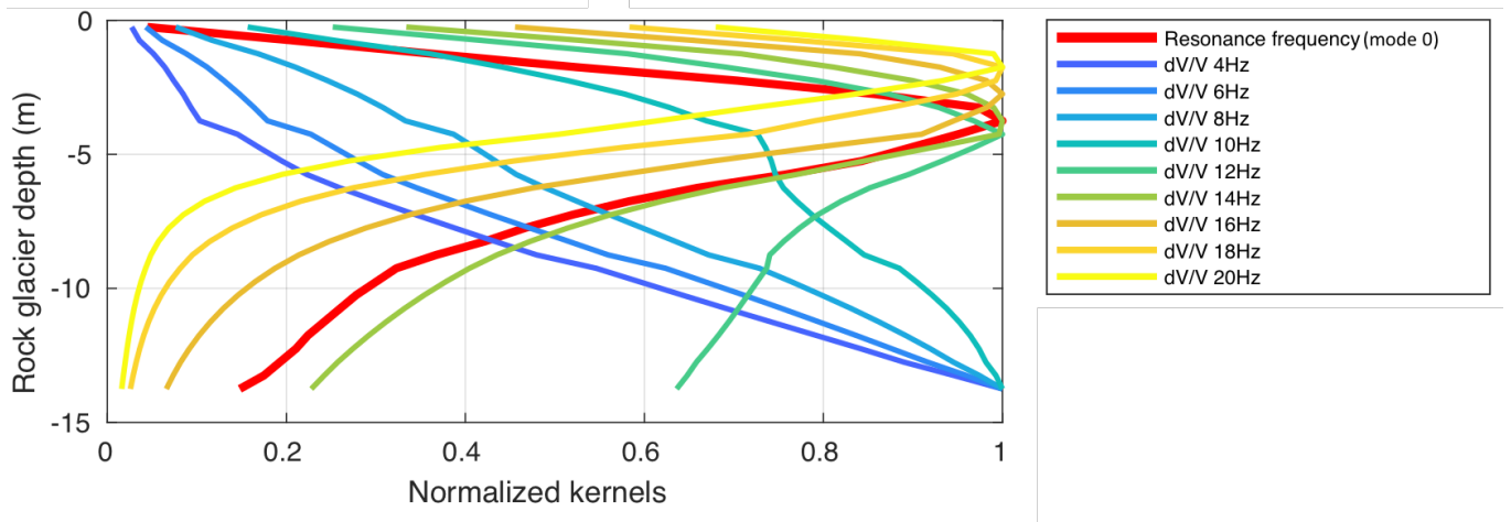
Figure 15 : Example of (normalized) depth sensitivity kernels of the two passive seismic methods for the Laurichard (C00 seismometer) rock glacier model. The red curve corresponds to the modal analysis (resonance frequency of the first vibrating mode). The other curves correspond to the ambient noise correlation (relative change of the Rayleigh wave velocity dV/V , depending of the frequency, shown by the other colours). At high frequencies ( > 14\text{Hz} ), dV/V is most sensitive at shallower depths than the resonance frequency of the first mode, whereas at low frequencies ( < 14\text{Hz} ), dV/V is most sensitive at deeper depths than resonance frequency.
