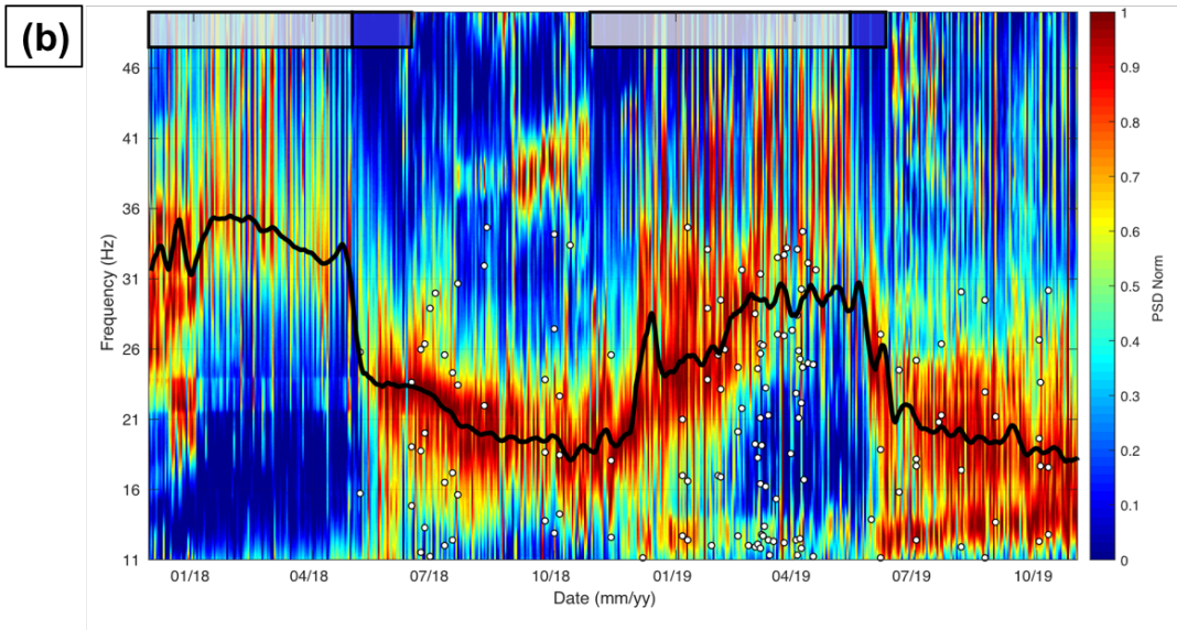
925 Figure 18: Normalized Power Spectra Density (PSD) from hourly spectrograms of the passive seismic recordings of Laurichard site, respectively from (a) C00 seismometer and from (b) C05 seismometer. The bold black line denotes the moving window average of hourly spectrogram maxima. For each recorded earthquake ( M > 2 ), the local maxima have been automatically picked (white dots) if it appears significantly on the spectrogram. Snow cover and melting periods are both figured by white and blue boxes above, respectively.
