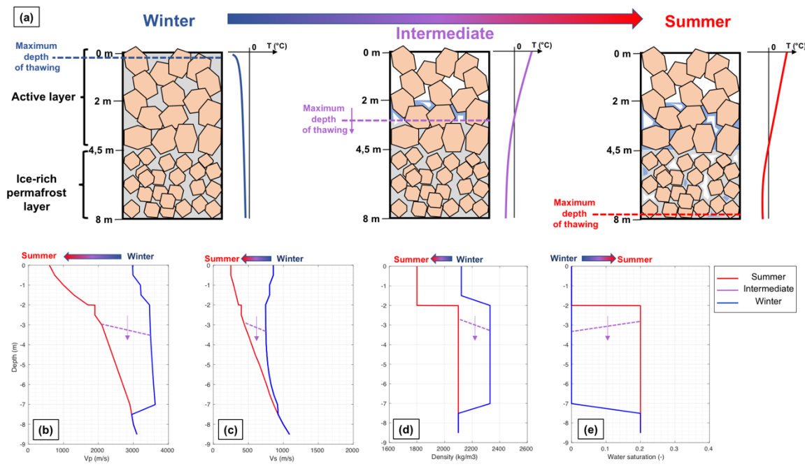
Figure 10: (a) Schematic cross-section of the Gugla rock glacier in winter (left) and in summer (right), and during the transition between them (intermediate state of thawing, in middle), as well as a schematic temperature profile associated with each of them, showing the main assumptions of the freezing modeling methodology by a poroelastic approach described in the text. The porous medium is composed of a rock matrix (in orange) and pores filled by water (in blue) or ice (in grey). With respect to the maximum depth of thawing varying from the surface to the ZAA depth, the evolution of parameters used by the model is respectively showed : P-wave velocity (b), S-wave velocity (c), the averaged density (d) and the water saturation (d). The values in summer are obtained from geophysics and boreholes, whereas the values corresponding to a frozen state (pores fully filled by ice, no more liquid water) are obtained by the 3-phases poroelastic model.
