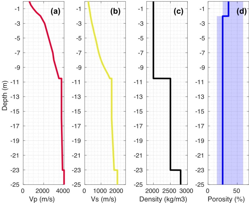
870 Figure 9 : Seismic velocity models of the Gugla rock glacier, based on geophysical investigations (seismic refraction) and from borehole data, with P-wave velocity (a) and S-wave velocity (b) profiles. The density (c) and the medium porosity ((d), solid blue curve) profiles are also shown, with low and high limits of the porosity used in the following mechanical modelling.
