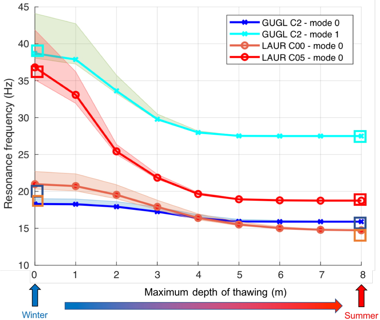
895 Figure 13: Results of the modal analysis for Gugla (GUGL) and Laurichard (LAUR) rock glaciers. The evolution of the resonance frequency of the respective synthetic modes is plotted, according to the maximal depth of thawing from the surface to the ZAA (8 m depth): left stands for the state of maximal freezing in winter (frozen medium until 8 m depth), right for the summer (unfrozen medium). The range of measured resonance frequency values is shown by the squares in the corresponding colors (estimated from Figure 3 and Figure 4 for respective sites). Errorbars (in transparency) show the influence of porosity on the results : the low (high) limit of errorbars shows the results for extremely low (extremely high) porosity profile.
