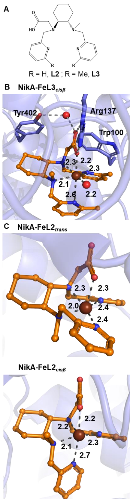
Figure 1. A: Structures of ligands L2 and L3 . B: Crystal structure of NikA-Fe L3 binding site. FeL3 under the only cisβ topology observed in this study. C: Crystal structure of NikA-Fe L2 binding site. FeL2 under either the trans or the cisβ topology, as observed in a previous study. [21] Fe is depicted as a brown sphere. Distances are in Å.
