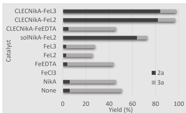
Figure 2. 1a oxidation by various catalysts under the following conditions: Catalyst:NaOCl: 1a : 1:255:600; [cat] = 37 μM in HEPES 10 mM pH 7; 2 hours except for CLEC [cat] = 31 μM in CH 3 CN:H 2 O 1/1 v:v ; 2 hours
