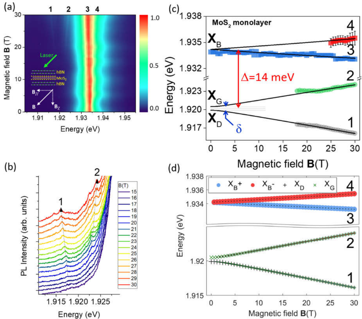
Figure 4 – Tilted (45°) magnetic field – The four mixed excitons states (labelled 1, 2, 3, 4) in MoS 2 monolayer revealed by magneto-photoluminescence. (a) Color map of the variation of the PL intensity as a function of B; (b) PL spectra for magnetic fields from 15 to 30 T showing the emergence of the two lowest energy states 1 and 2 (mainly with grey and dark components). (c) Magnetic field dependence of the energy of the four mixed exciton states. The full lines are fits to the model described in the text. The notations dark exciton (X D ), grey exciton (X G ) and bright excitons (X B ) are only strictly valid at 0 T. (d) Same fitting results than in (c). The size of each symbol is proportional to the weight of each component (the two bright component X B + and X B - and the two dark component X G and X D ) (See S18 for the calculation of the weight of the four components at high field).
