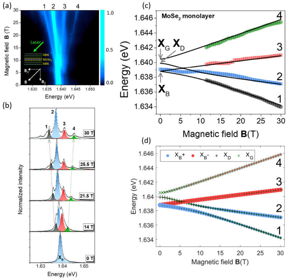
Figure 3 – Tilted (45°) magnetic field – The four mixed exciton states (labelled 1, 2, 3, 4) in MoSe 2 monolayer revealed by magneto-photoluminescence. (a) Color map of the variation of the PL intensity as a function of B ; (b) PL spectra for magnetic fields from 0 to 30 T showing the emergence of the four mixed states (the intensity is normalized to the main exciton line (state 2)). (c) Magnetic field dependence of the energy of the four mixed exciton states. The full lines are fits to the model described in the text. The notations dark exciton ( X_D ), grey exciton ( X_G ) and bright excitons ( X_B ) are only strictly valid at 0 T. (d) Same fitting results than in (c). The size of each symbol is proportional to the weight of each component (the two bright component X_B^+ and X_B^- and the two dark component X_G and X_D ) (See S18 for the calculation of the weight of the four components at high field).
