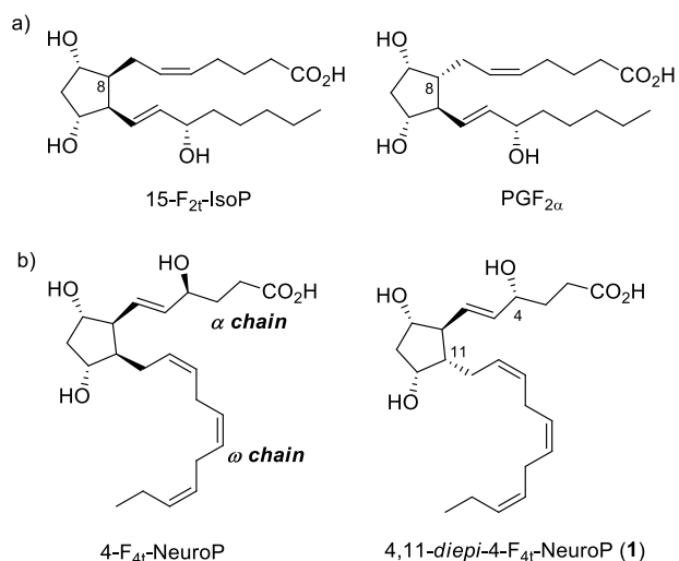
Figure 1. (a) PGF 2α and its C8 epimer (15-F 2t -IsoP). (b) Structures of 4-F 4t -neuroprostane and 4,11- diepi -4-F 4t -neuroprostane ( 1 ). By definition, the \alpha chain in PGs has to be presented on top.
