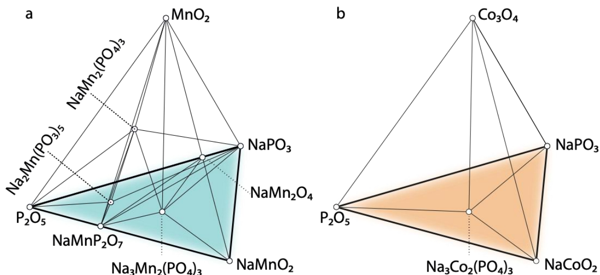
Figure 7 Panels a and b show portions of the computed phase diagrams of Na-P-O-Mn and Na-P-O-Co at 0 K. Two stable NaSICON structures, i.e., \text{NaMn}_2(\text{PO}_4)_3 and \text{Na}_3\text{Mn}_2(\text{PO}_4)_3 are observed in the phase diagram of Na-P-O-Mn, which are in equilibrium with the highly stable binary ( \text{P}_2\text{O}_5 and \text{MnO}_2 ) and ternary ( \text{NaMnO}_2 and \text{NaPO}_3 ) compounds. In panel b , a stable NaSICON structure, i.e., \text{Na}_3\text{Co}_2(\text{PO}_4)_3 is observed in the phase diagram of Na-P-O-Co, which is in equilibrium with the highly stable binary ( \text{P}_2\text{O}_5 and \text{Co}_3\text{O}_4 ) and ternary ( \text{NaCoO}_2 and \text{NaPO}_3 ) compounds.
