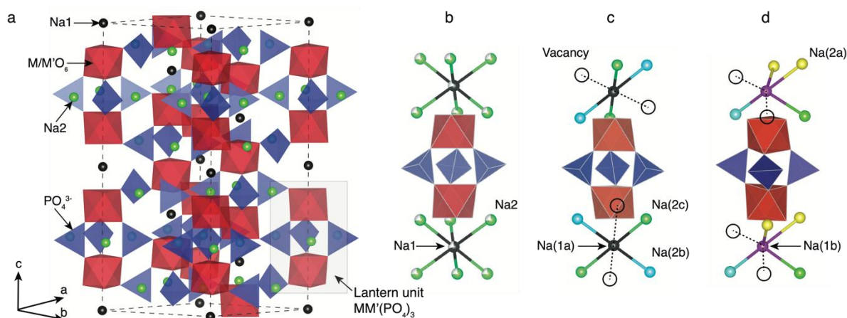
Figure 1 a The rhombohedral ( R\bar{3}c ) structure of \text{Na}_4\text{MM}'(\text{PO}_4)_3 with M and M' = \text{Ti, V, Cr, Mn, Fe, Co} and \text{Ni} . The “lantern unit” is made up of two \text{MO}_6 (or \text{M}'\text{O}_6 ) octahedra (red) sharing corners with \text{PO}_4^{3-} tetrahedra (blue). The gray box in (a) highlights the arrangement of lantern units. Two distinct Na ions, i.e., Na1 (black) and Na2 (green), are present in the rhombohedral NaSICONs. Panel b lantern representation of the Na disordering (with partial Na occupancies on Na1 and Na2 sites) in the rhombohedral \text{Na}_3\text{MM}'(\text{PO}_4)_3 polymorph. Panel c shows a local view (lantern unit) of the complete ordering of \text{Na}^+ ions in the corresponding \text{Na}_3\text{MM}'(\text{PO}_4)_3 monoclinic ( C2/c ) phase. Panel d shows the local environment of sites Na1b (violet) and Na2a (yellow) in the same monoclinic arrangement. Vacancies are represented by open circles.
