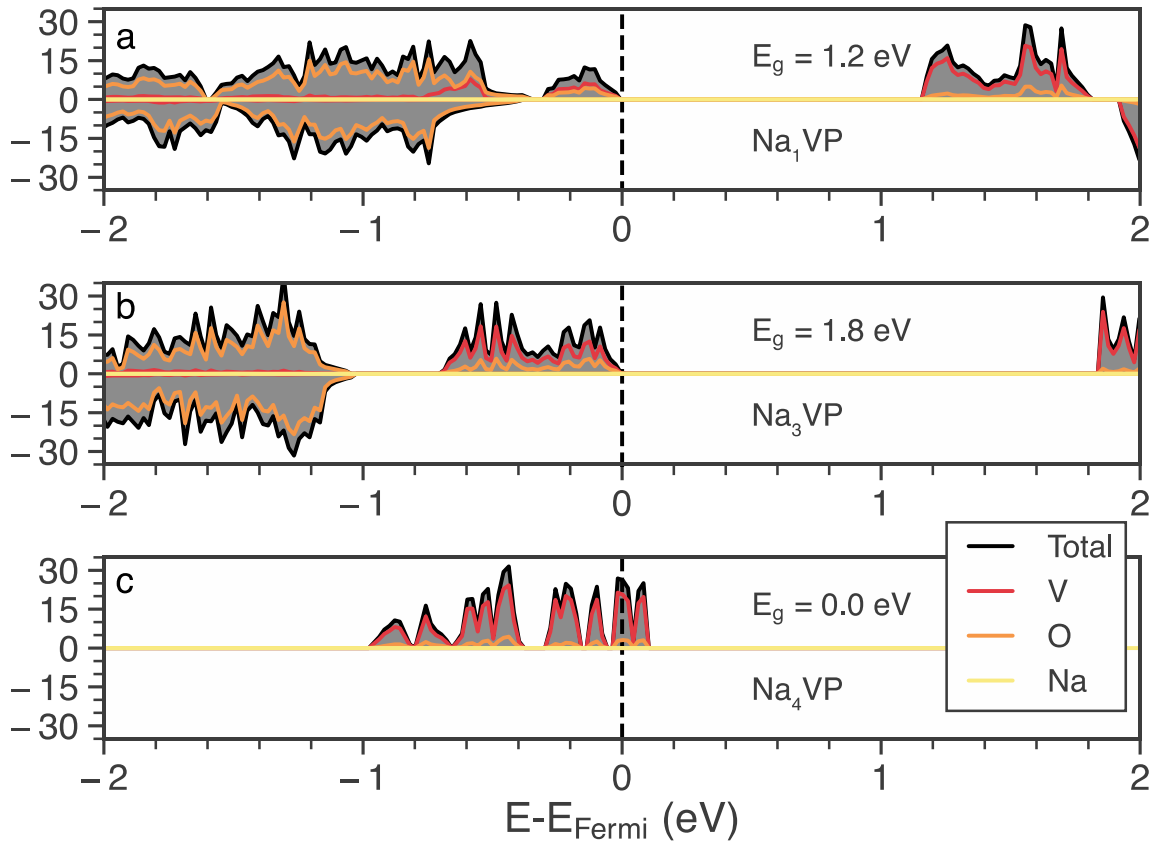
Figure 3 The total (gray) and atom projected (V red, O orange and Na yellow) DOS of \text{Na}_x\text{V}_2(\text{PO}_4)_3 NaSICON (NVP), where for Na concentrations x = 1, 3 and 4 . The vertical line denotes the Fermi energy level and E_g is the calculated band gap at the GGA+ U level of theory.
