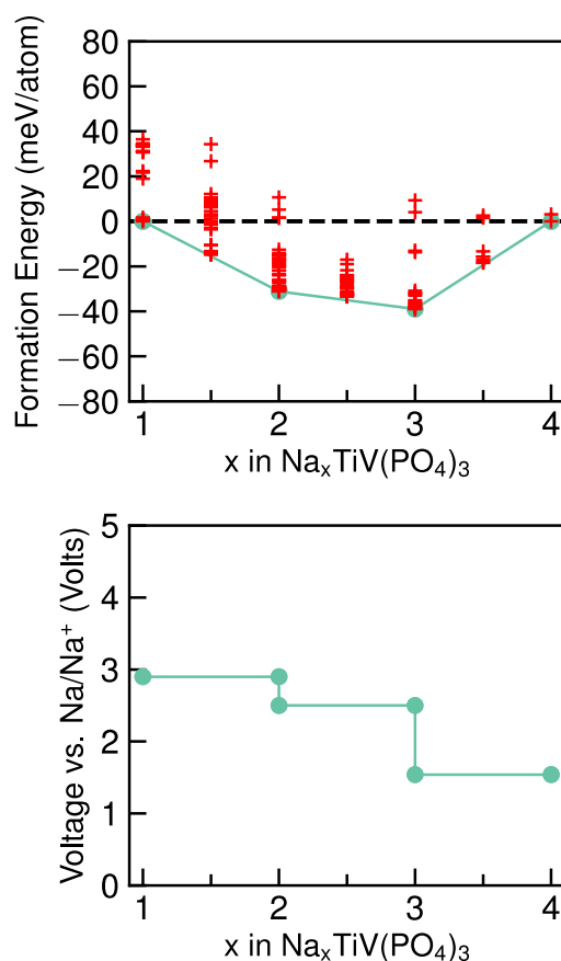
Figure S13 (upper panel) The computed formation energies and respective convex hulls (green line) for Na vacancy orderings as a function of Na concentration ( x ) in \text{Na}_x\text{TiV}(\text{PO}_4)_3 . (lower panel) The corresponding intercalation voltage vs. \text{Na}/\text{Na}^+ at different Na content. Note that x varies in the range 1 \leq x \leq 4 . The stable orderings forming the convex hull are displayed as green dots while the unstable orderings are given as red symbols.
