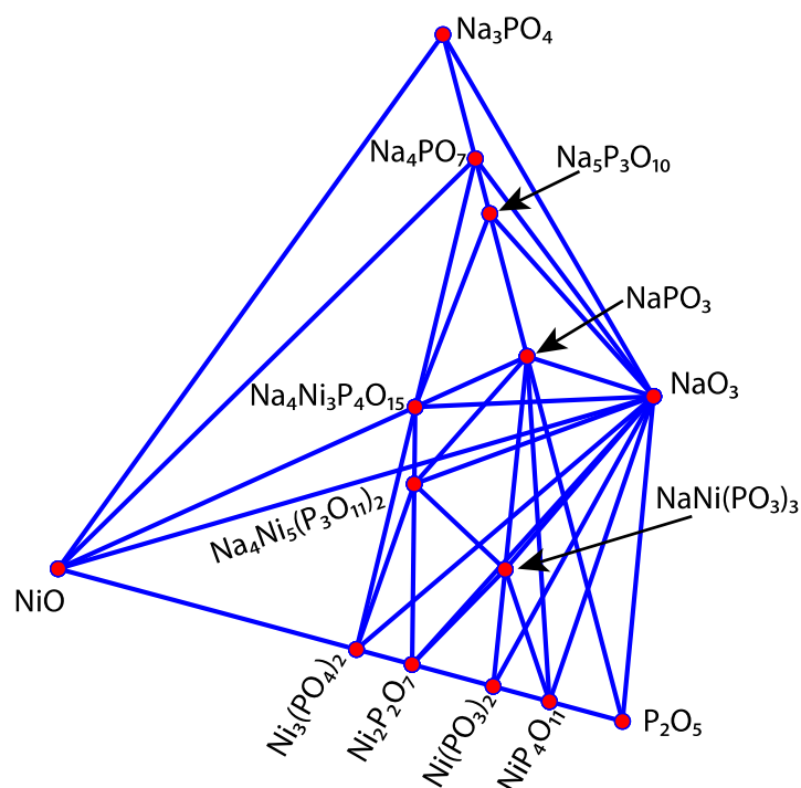
Figure S34 The computed phase diagram of chemical system Ni-Na-P-O at 0K. No stable NaSICON structures with formula \text{Na}_x\text{Ni}_2(\text{PO}_4)_3 was observed in the global phase diagram. The compounds with compositions close to NaSICON are plotted which is in equilibrium with highly stable binaries ( \text{P}_2\text{O}_5 , NiO and \text{NaO}_3 ) and ternaries ( \text{Na}_3\text{PO}_4 ).
