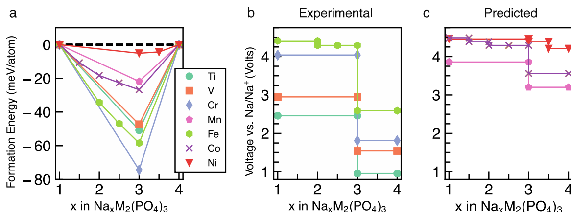
Figure 2 Panel a shows the computed formation energies and respective convex hulls for Na vacancy orderings as a function of Na concentration ( x ) in \text{Na}_x\text{M}_2(\text{PO}_4)_3 where M = \text{Ti}, \text{V}, \text{Cr}, \text{Mn}, \text{Fe}, \text{Co} and \text{Ni} . Panels b and c show the intercalation voltages vs. \text{Na}/\text{Na}^+ for the experimentally known ( M = \text{Ti}, \text{V}, \text{Cr} and \text{Fe} ) and predicted ( M = \text{Mn}, \text{Co} and \text{Ni} ) \text{Na}_x\text{M}_2(\text{PO}_4)_3 compounds, respectively. Only the stable orderings forming the convex hull are displayed in panel a . The energies of unstable configurations for each convex hull are shown in Figures S1-S7 of the SI.
