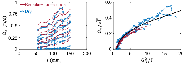
FIG. 4. Comparison to LEFM predictions for rupture velocities approaching C_R . (Left) Maximal material velocities \dot{u}_x measured at points (l, y = 3.5 \text{ mm}) for the ruptures presented in Fig. 3. (Right) Collapse of these measurements is obtained, as described by LEFM, when \dot{u}_x amplitudes are plotted with respect to G_{II}^S/\Gamma and scaled by \sqrt{\Gamma} . Note that \dot{u}_x amplitudes span 2 orders of magnitude and increase significantly as C_f \rightarrow C_R . The solid line designates the values predicted by LEFM. The values of \dot{u}_x provide a more detailed comparison with LEFM than the equation of motion for C_f \rightarrow C_R as occurs for G_{II}^S \gg \Gamma .
