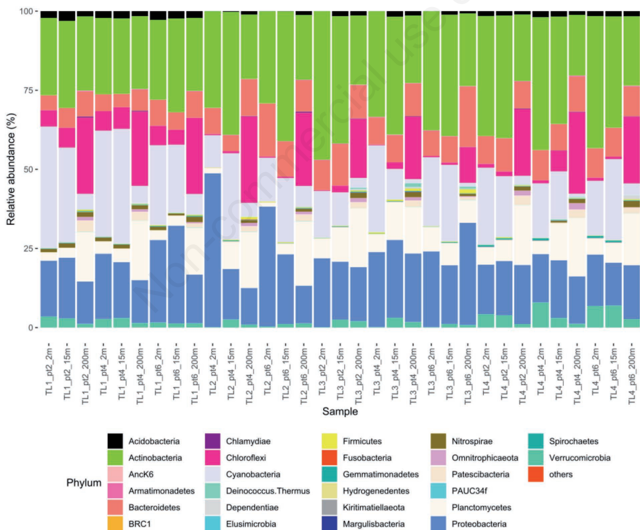
Fig. 4. Stacked histogram of bacterial phylum. Phylum abundances are represented by read relative abundance per sample. Phyla with less than 5% of read relative abundance in a sample are merged and identified as “others”.
