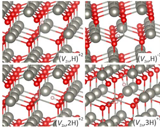
Figure 4. Structural models for the most stable atomic configurations of each of (V_{\text{Zn}},\text{H})^{+2} , (V_{\text{Zn}},\text{H})^{-1} , (V_{\text{Zn}},2\text{H})^{+2} , and (V_{\text{Zn}},3\text{H})^{+1} defect complex. Large grey balls denote Zn atoms, small red balls denote oxygen atoms and small white balls denote hydrogen atoms. The Zn atom in front of the V_{\text{Zn}} was removed for the sake of clarity and only its bonds with the neighboring oxygen atoms are presented.
