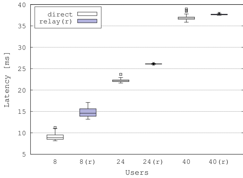
Figure 13: Boxplot of latency of VoIP flows
