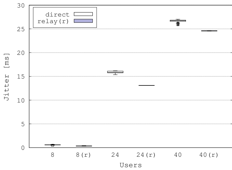
Figure 14: Boxplot of jitter of VoIP flows
