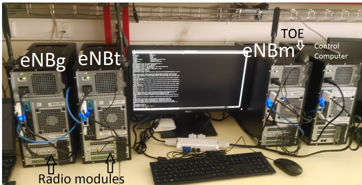
Fig. 3: Implementation of the test-bed
