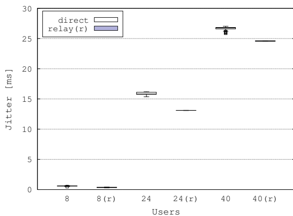
Fig. 14: Boxplot of jitter of VoIP flows
