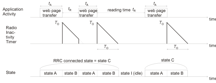
Fig. 5: Illustration of activity and reading times
