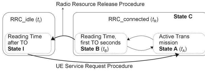
Fig. 6: Activity model with related RRC states
