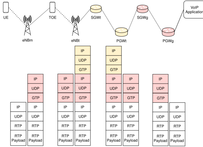
Fig. 8: VoIP packet headers in relay architecture.
