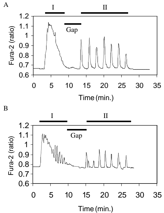
Fig. 1. (A,B) Examples of sperm-triggered Ca 2+ oscillations at fertilization in different egg batches. (A) Unfertilized denuded ascidian eggs were injected with Fura-2 dextran to give an intracellular concentration of approximately 20 µM. The eggs were then fertilized and the Ca 2+ oscillation pattern triggered by sperm recorded at 5 second intervals for a period of 35 minutes. (A) Sperm trigger two phases of Ca 2+ oscillations (I and II) separated by a gap. (B) In addition to the pattern observed previously in A, there are a number of Ca 2+ oscillations during the first phase (labelled I). Again there is a short gap phase before the second phase of Ca 2+ oscillations are generated (n=28). Temperature, 19°C.
