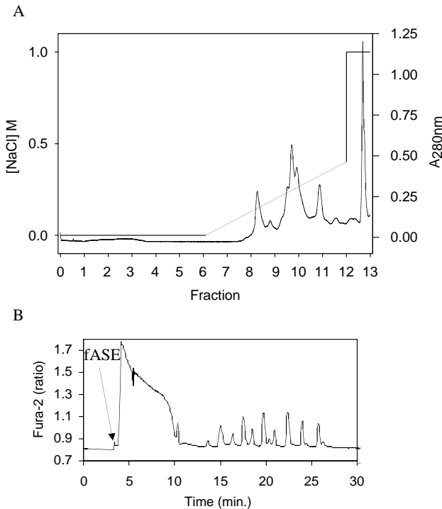
Fig. 5. Fractionation of ascidian sperm extract. (A) Ascidian sperm extract was desalted then applied to a MonoQ column at pH 8.5, eluted with an increasing gradient of NaCl and 2 ml fractions collected. Fractions 1-3 contain the material that did not bind to the column. (B) Injection of fraction 11 into an unfertilised ascidian egg (fASE at the arrow) containing approximately 20 μM Fura-2 dextran triggers two series of Ca 2+ oscillations that terminate at the end of meiosis (9/9). The first Ca 2+ signal is larger than that seen with ASE and is initiated sooner after injection, which may indicate a concentration of the ASE through fractionation.
