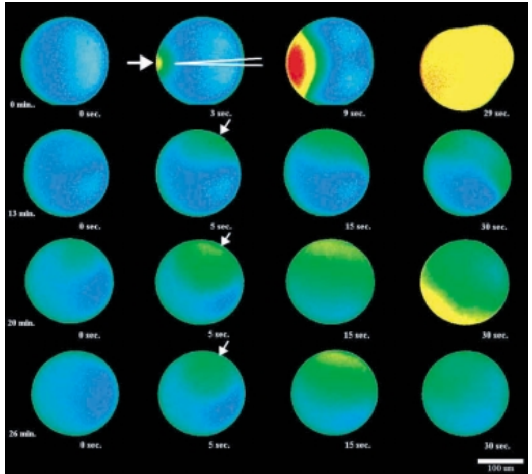
Fig. 3. ASE triggers a series of \text{Ca}^{2+} oscillations that mimic fertilization spatially. The pseudocolour images represent the ratio signal generated by the Fura-2 emission. Unfertilised denuded ascidian eggs contained approximately 20 \mu\text{M} Fura-2 dextran before injection of ASE. The figure shows a single egg at various times after injection. The animal pole was located at the point indicated by the large arrow. The injection pipette was introduced into the egg as indicated (although at this time the injection pipette had already been removed). Injection of ASE (0.1–0.2%) resulted in a rapid increase in \text{Ca}^{2+} levels near the site of injection (34 seconds following injection in this particular egg). About 29 seconds after the first [\text{Ca}^{2+}] increase the cortical contraction is visible. Note the large bulge at 2 o'clock. The eggs are slightly wedged so occasionally rotate slightly. Once the contraction has ceased and the \text{Ca}^{2+} levels have returned to basal values the egg enters the gap phase. The [\text{Ca}^{2+}] increases again 13 minutes after the first [\text{Ca}^{2+}] increase. Three \text{Ca}^{2+} waves are displayed originating from the same site (small arrow). This site is far from the site of origin and was confirmed to be equivalent to the contraction pole area ( n=8 ). Cooler colours represent basal \text{Ca}^{2+} levels (blue-green) and warmer colours (yellow to red) represent increasing \text{Ca}^{2+} levels. Temperature, 19°C.
