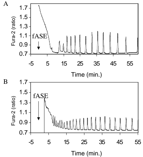
Fig. 6. Cyclin-dependent kinase (CDK) activity and not the MAP kinase activity controls the Ca 2+ oscillations initiated by fASE. (A) Unfertilised ascidian eggs were injected with mRNA encoding Δ90 cyclin B1, left for 3 hours to produce Δ90 cyclin B1 protein (determined by fluorescence emission) and then injected with Fura-2 dextran (approximately 20 μM). fASE was then injected and the Ca 2+ oscillations monitored. Injection of fASE at the arrow triggers a series of Ca 2+ oscillations that do not stop during a 60 minute observation period (4/4). (B) Batches of eggs containing Δ90 cyclin B1 and Fura 2-dextran were incubated in 10 μM U0126 for 20 minutes then injected with fASE at the arrow. The Ca 2+ oscillations were monitored for a 60 minute period, and again the Ca 2+ oscillations triggered by fASE did not stop during the period of observation (4/4). Temperature, 19°C.
