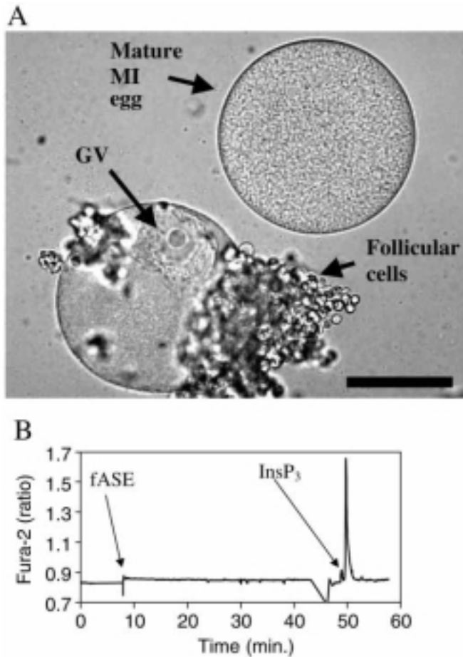
Fig. 7. fASE does not trigger \text{Ca}^{2+} release in prophase-stage oocytes. (A) A prophase-stage oocyte that was previously injected with fASE and then \text{InsP}_3 , together with a mature egg. The nucleolus is clearly visible inside the large germinal vesicle (GV). There are some follicular cells attached to the prophase-stage oocyte. Bar, 100 \mu\text{m} . (B) Prophase-stage oocytes were microinjected with Fura-2 dextran (to give approximately 20 \mu\text{M} in the cytosol) and subsequently injected with a supramaximal dose of fASE (approx. 0.5%). This did not trigger any \text{Ca}^{2+} release in a 30 minute period of observation (4/4). Subsequent injection of \text{InsP}_3 did trigger a \text{Ca}^{2+} release (0.1% injection, 100 nM in the oocyte, 3/3). It was confirmed that fASE was capable of triggering \text{Ca}^{2+} oscillations in a mature egg from the same batch (data not shown). MI, metaphase I. Temperature, 19°C.
