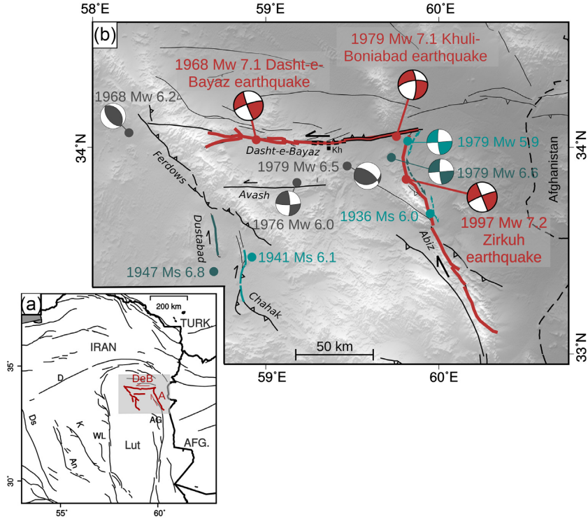
Figure 1. Regional tectonic overview and the NE Lut earthquake sequence. (a) Map of eastern Iran showing the main tectonic faults (thin black lines) and the study area in (b) (light grey box). The faults involved in the NE Lut sequence are highlighted in red. Ds, An, K, D, WL, DeB, A and AG mean Deshir, Anar, Kuhbanan, Doruneh, West Lut, Dasht-e-Bayaz, Abiz and Avaz-Gazik faults, respectively. Fault mapping is from Walpersdorf et al. (2014). TURK and AFG are for Turkmenistan and Afghanistan. (b) Topographic map of northeastern Iran showing the epicentres of the 11 events of the NE Lut sequence (dots). The epicentres of historical earthquakes (pre-1968) are from Ambraseys & Melville (1982) and those of instrumental earthquakes are from Engdahl et al. (2006). M_w > 7 earthquakes and their surface rupture are plotted in red whereas moderate earthquakes ( 5.9 < M_w < 7 ) and their surface rupture are plotted in blue. Fault names are written in italic and the black square locates the city of Khuli (Kh). The surface ruptures of the Dasht-e-Bayaz and the Khuli-Boniabad earthquakes overlap near Khuli (dashed black line). The double dotted arrows indicate the surface rupture extent of the three moderate earthquakes that broke the Abiz fault. No surface rupture has been reported for the earthquakes plotted in grey. The 1979 M_w 6.5 event has broken an unmapped fault.
