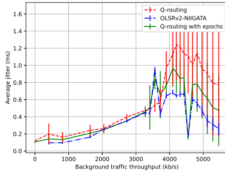
Figure 7: Average jitter on the toy example (scenario 2).
