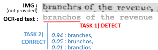
Fig. 1. Two tasks: error detection and error correction.
