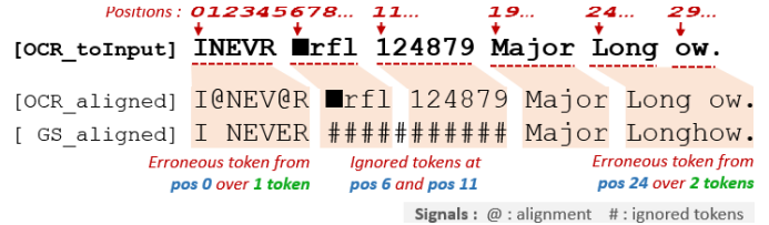
Fig. 2. Sample of the training set provided to the participants.
