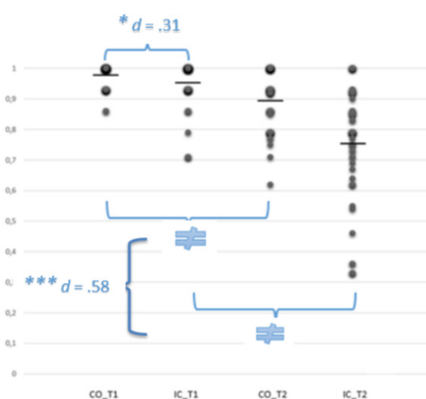
Figure 1: Participants' accuracy scores on congruent (CO) and incongruent (IC) items without time restriction (T1) and with time restriction (T2). Vertical stripes indicate the mean score.
