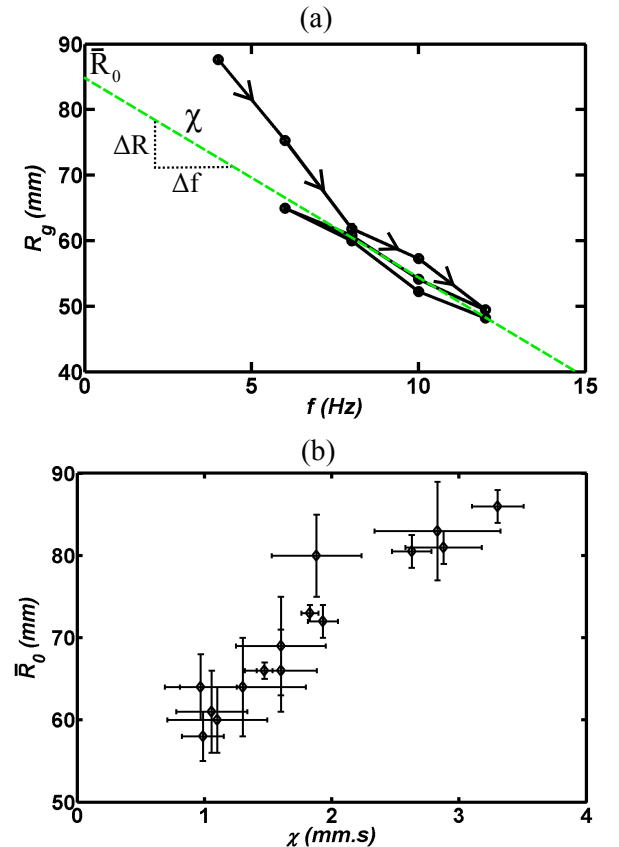
FIG. 5: Susceptibility. (a) Evolution of the radius of gyration R_g during an annealing experiment. After a first irreversible brach, the radius follows a reversible branch (parallel to the dashed line). A configuration is characterized by the slope of the line, \chi , and its intercept, R_0 , with the axis f = 0 . (b) The characteristic radius R_0 as a function of susceptibility \chi . Each point corresponds to one realization of an annealing experiment. The error bars correspond to the uncertainties estimates of the linear fits as described in (a).
