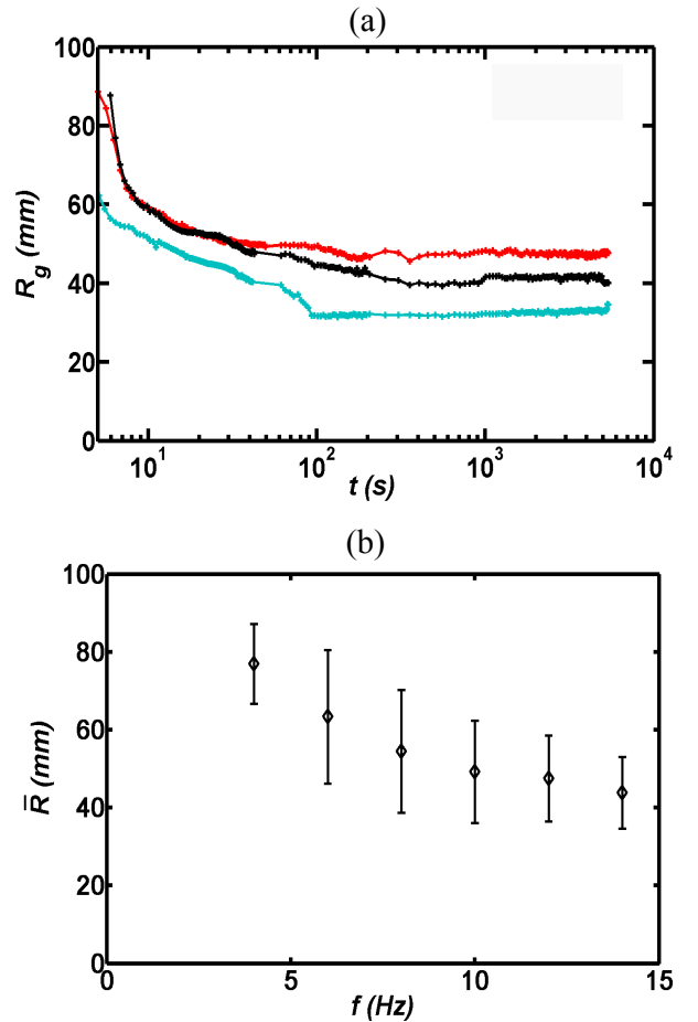
FIG. 3: The radius of gyration. (a) The radius of gyration R_g as a function of time for three realizations in which the cell was launched from 0 to 14 Hz in 3 s. Radii reach a plateau value in about 10^3 s. The final radius differs according to realizations. (b) On average, the radius of gyration \bar{R} decreases with the strength of confinement (quantified by the rotation velocity, f of the disk). Bars represent the width of radii distribution for a given rotation frequency.
