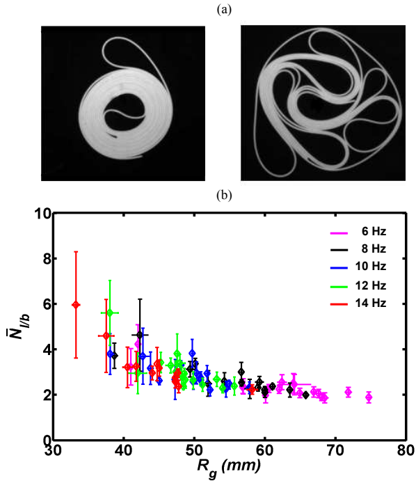
FIG. 4: Stacking. (a) Order and disorder. Two extreme examples of equilibrium configurations obtained at two different frequencies, with a large and a small number of superposed layers, respectively. (b) Average number of layers per branch, N_{l/b} , as a function of the radius of gyration R_g . Each point corresponds to one realization of the experiment. The colors of the symbols correspond to the imposed rotation velocity of the disk. An ordered configuration (large N_{l/b} ) has a small radius of gyration.
