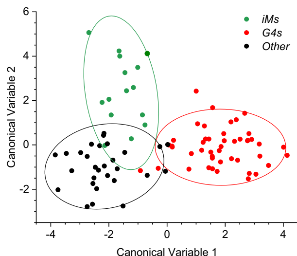
Figure 8. Canonical variable 1 versus Canonical variable 2 plot obtained from LDA of the reduced emission dataset (normalized emission data recorded at 335, 338, 341, 380, 383 and 386 nm in buffer A, and 329, 332, 376, 379, 382, 385, 388 and 391 nm in buffer B, \lambda_{\text{ex}} = 260 nm) on 89 characterized sequences. Ellipses represent 85% confidence zones for each group.
