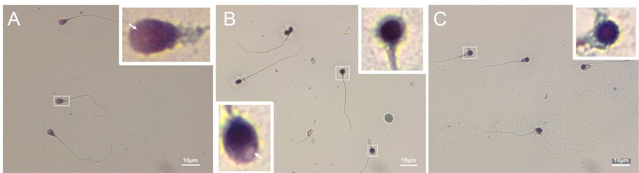
Fig. 1 Optical microscopic observations of spermatozoa. Scale=10 \mu M. The acrosome is at the tip of the white arrow. a Semen of a control patient with only normal spermatozoa (absent from the cohort). Zoom on a spermatozoon's head of typical shape (white square in the upper right corner). The acrosome can be identified as the white halo at the front of the head. The nucleus is the black part closer to the intermediate piece. b Semen from a patient with partial globozoospermia. Zoom on a round headed spermatozoon
