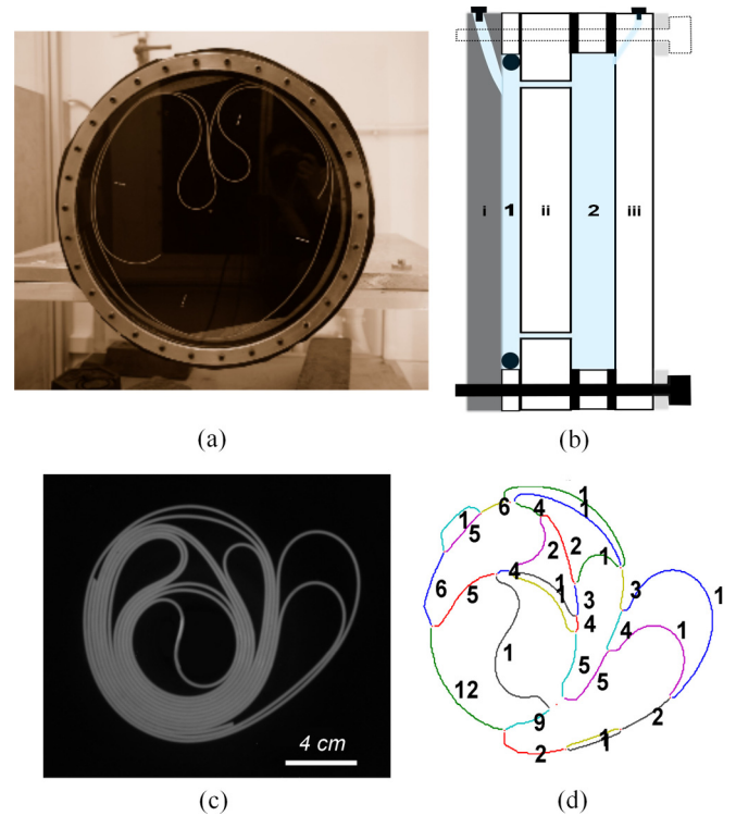
FIG. 1. (Color online) The experiment. (a) A rod of density 1 g/cm 3 is confined in a circular Hele-Shaw cell, filled with salt-saturated water of density 1.16 g/cm 3 . (b) The cell is made of a superposition of three disks; the intermediate one (ii) is pierced with two holes to enable equilibration of pressure into the liquid. This setup enables the fixing of the thickness of chamber 1 where the rod is placed, chamber 2 being a sacrificial room. The chambers are made watertight with flat and toric joints shown in black. (c) Example of an equilibrium configuration obtained when a centripetal force is generated by the rotation of the cell around its axis. (d) Corresponding skeletonized image in which the number of layers per branch is defined. Figure reproduced from [33].
