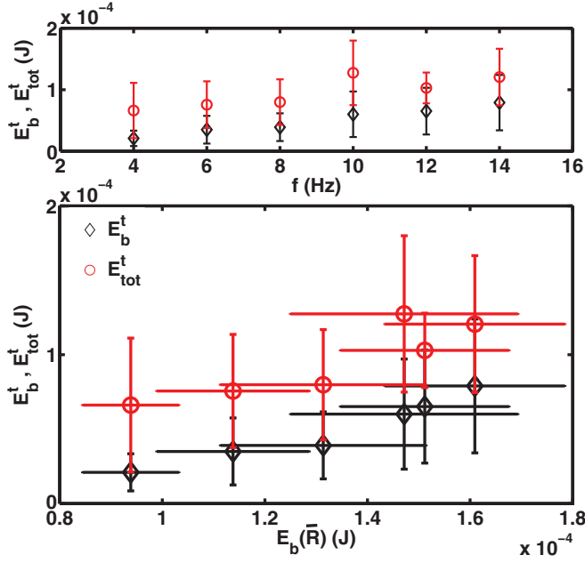
FIG. 7. (Color online) The energy scales E_b^t ( \diamond ) and E_{tot}^t ( \circ ) as functions of the rotation frequency f (top) and as functions of the bending energy of a ring of radius \bar{R}(f) given by Eq. (7) (bottom).
