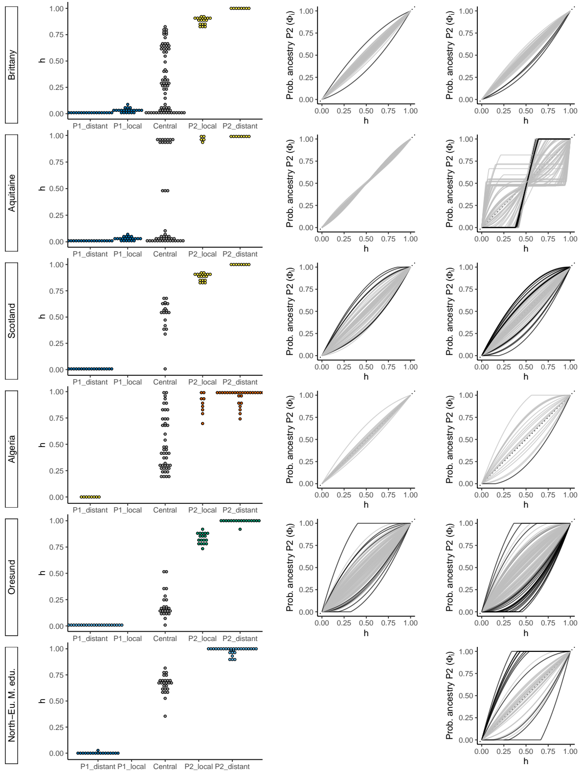
Figure 5: Left panels: Hybrid index ( h ) distributions from introgress, for each group of the hybrid zone. middle panels: Genomic cline computed with the local parental groups (P1_local, P2_local or distant when not available) with cline presenting a significant excess in either \alpha or \beta parameters highlighted in black. right panels: Genomic cline computed with distant populations as parental groups. For genomic cline, only markers with an allele frequency difference > 0.3 between P1_distant and P2_distant are drawn. The probability of the locus-specific ancestry for P2 against the genome wide hybrid index ( h ) is plotted. When distant parental populations are used in place of local ones, the number of discordant loci increases. See Table 3 for a list of the populations used in the analyses.
