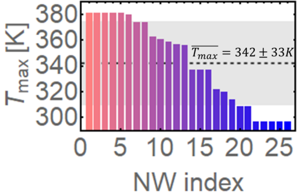
FIG. 4. Maximum lasing operation temperature of 26 different NWs. The horizontal dashed line and grey shading represent the mean \overline{T_{max}} = 342K and the standard deviation 33K of the maximum operation temperature for the set of 26 NWs.
