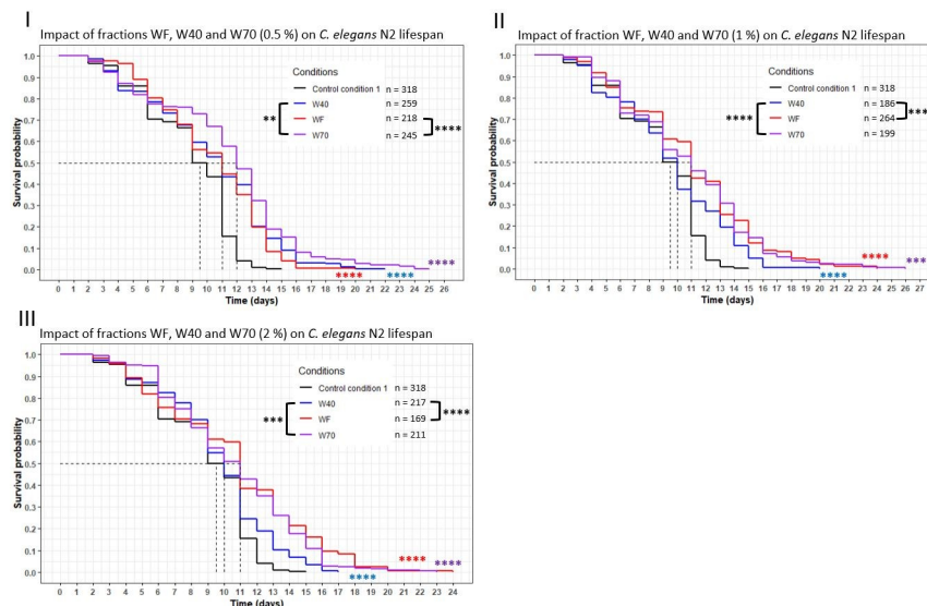
Fig 5. Comparison of the effect of aqueous fractions WF, W40 and W70 on C. elegans wild-type N2 strain lifespan. Worms were incubated on aqueous fractions at day 0 and fed every three days with OP50 HK. The asterisks indicate the p -values (log-rank test) (“*” p < 0.05; “**” p < 0.01; “***” p < 0.001; “****” p < 0.0001). The asterisks around the curves are the comparisons with the control conditions. The asterisks around the legend are the comparisons between the fractions.
