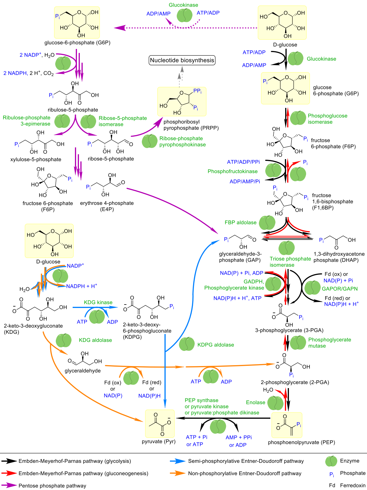
Figure 7. An overview of biological carbohydrate synthesis and breakdown. 90,139 Only key intermediates and enzymes are shown. Major biochemical hubs are highlighted by yellow boxes.
