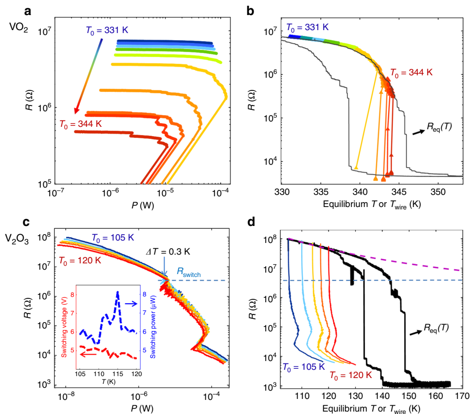
Fig. 2 Thermal vs. non-thermal IMT switching. a and c R(P) curves acquired at different substrate temperatures, T_0 , corresponding to the insulating state of VO 2 and V 2 O 3 nanowires, respectively. The IMT switching is manifested as abrupt resistance jumps. b and d R(T_{\text{wire}}) curves derived from the corresponding R(P) curves and superimposed on the R_{\text{eq}}(T) (black). For the VO 2 nanowire in b , the excellent correspondence between R(T_{\text{wire}}) and R_{\text{eq}}(T) signifies that the IMT is triggered thermally. For the V 2 O 3 nanowire in d , no such correspondence between R(T_{\text{wire}}) and R_{\text{eq}}(T) is observed, showing the inadequacy of a Joule-heating driven mechanism. The IMT switching in c begins with an increase of temperature \Delta T = 0.3 \text{ K} in T_{\text{wire}} regardless of T_0 (light blue arrow), indicating a negligible role of Joule heating. The switching resistance R_{\text{switch}} (dashed blue line) is lower than the fully insulating state resistance at any temperature. This is shown in d by the extrapolation of R_{\text{eq}}(T) according to thermally activated resistance behavior with an activation energy of 60 meV (purple dashed line). The inset in c shows the switching voltage and power as functions of T_0 .
