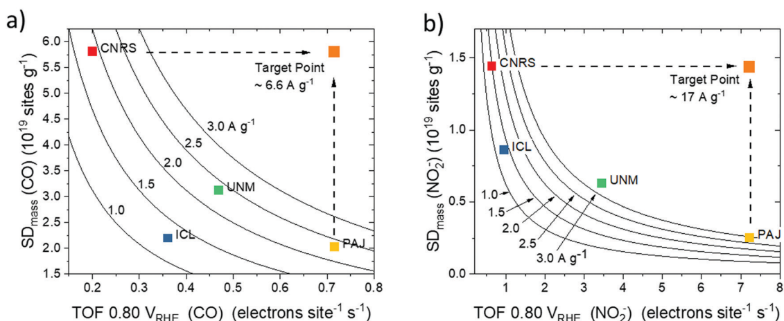
Fig. 6 Site density–ORR turnover frequency maps ( SD – TOF ORR reactivity maps) obtained by plotting the Fe surface site density ( SD ) and the corresponding TOF for each of the four catalysts with iso-mass activity hyperbolic curves at 0.80 V_{\text{RHE}} : (a) SD – TOF reactivity map derived from SD_{\text{mass}}(\text{CO}) (pH 1, activity values from Table 1) and (b) SD – TOF reactivity map derived from SD_{\text{mass}}(\text{NO}_2^-) (pH 5.2 Fig. S9–S12, ESI†). SD – TOF reactivity maps allow for a rational deconvolution and analysis of ORR reactivity of PGM-free catalysts. They also aid in establishing fundamental synthesis–reactivity relationships. Dashed arrows indicate examples of catalyst target performance superimposing the highest observed SD (CNRS) with the highest observed TOF (PAJ).
