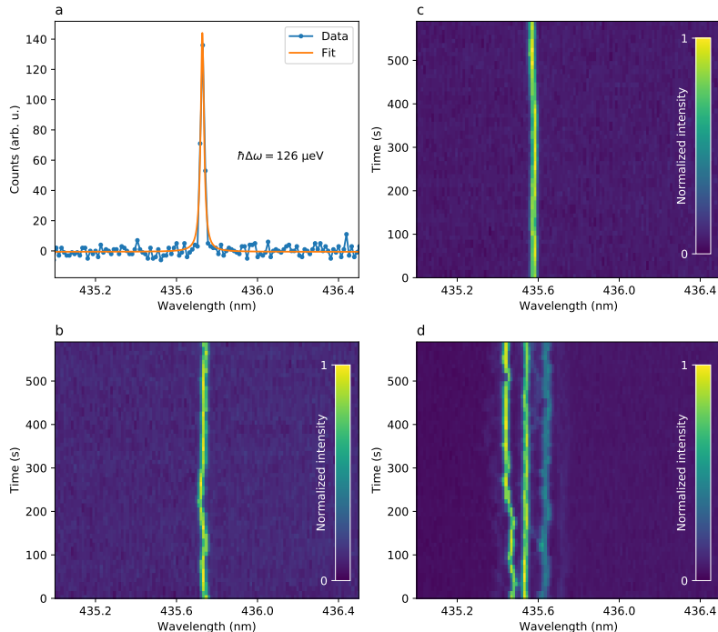
Figure 4: Spectral properties of individual SPEs at low temperature (5 K). (a) High-resolution spectrum of SPE 1 ZPL, showing a resolution-limited line at 435.73 nm (b) Spectral diffusion of SPE 1 ZPL during 600 s. The standard deviation of the centre wavelength over time is found to be 45 \mu\text{eV} , as determined by Lorentzian fits of the data. (c) Spectral diffusion of another SPE (SPE 2 ) and (d) spectral diffusion of an ensemble of three SPEs, with uncorrelated fluctuations of different magnitudes. All SPEs are excited with 1 mW cw laser light at 405 nm.
