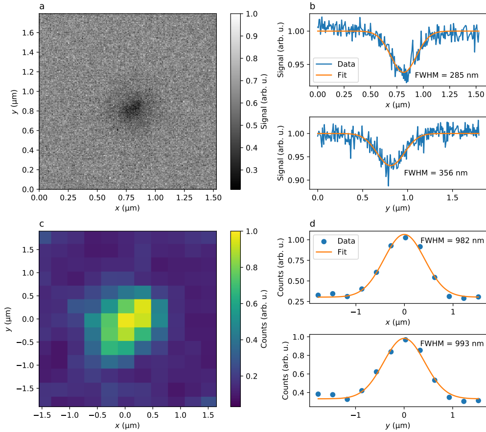
Figure 1: (a) SEM image of an irradiation on the \text{SiO}_2 substrate. (b) Sum along x (upper panel) and y (lower panel) from which we estimate the beam dimensions. The orange lines are Gaussian fits of the data. (c) Room temperature photoluminescence confocal map of a SPE ensemble from an irradiation spot. (d) Cuts along x (upper panel) and y (lower panel) from which we extract the characteristic dimensions of the SPE ensemble.
