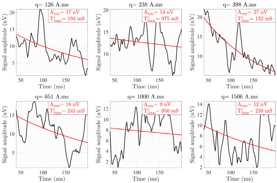
Fig. 6. Recorded signal at station 6.
