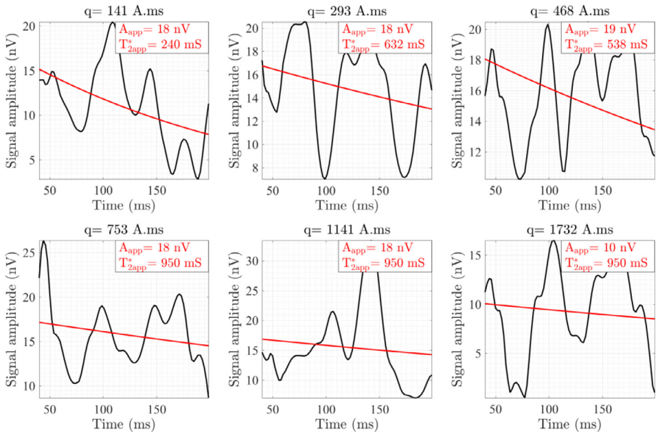
Fig. 14. Recorded signal at station 16.
