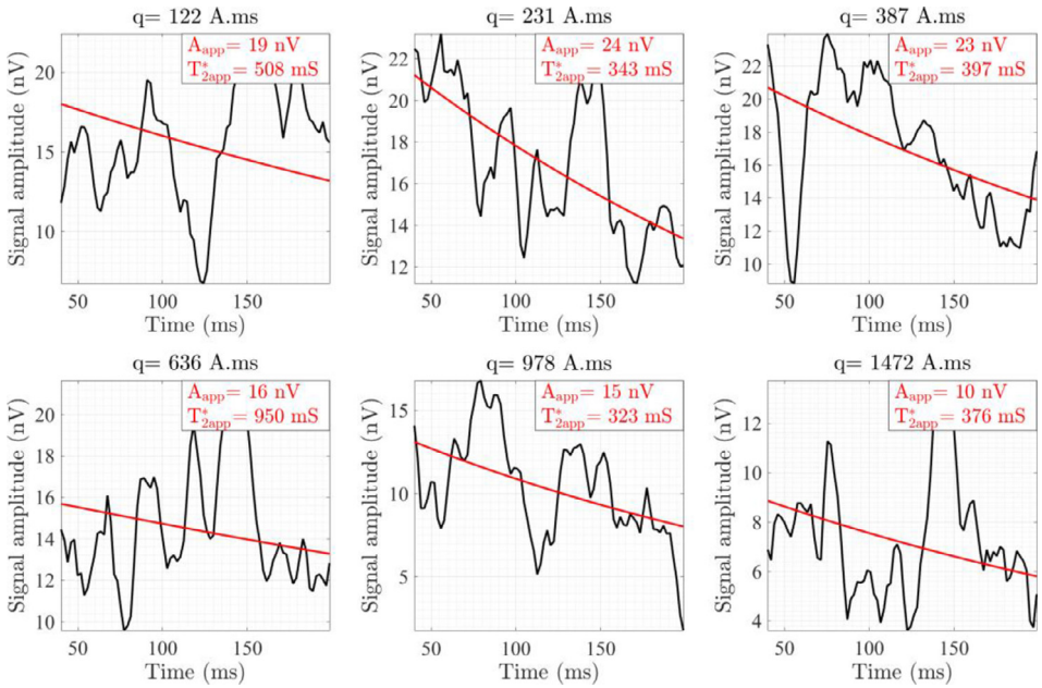
Fig. 10. Recorded signal at station 12.
