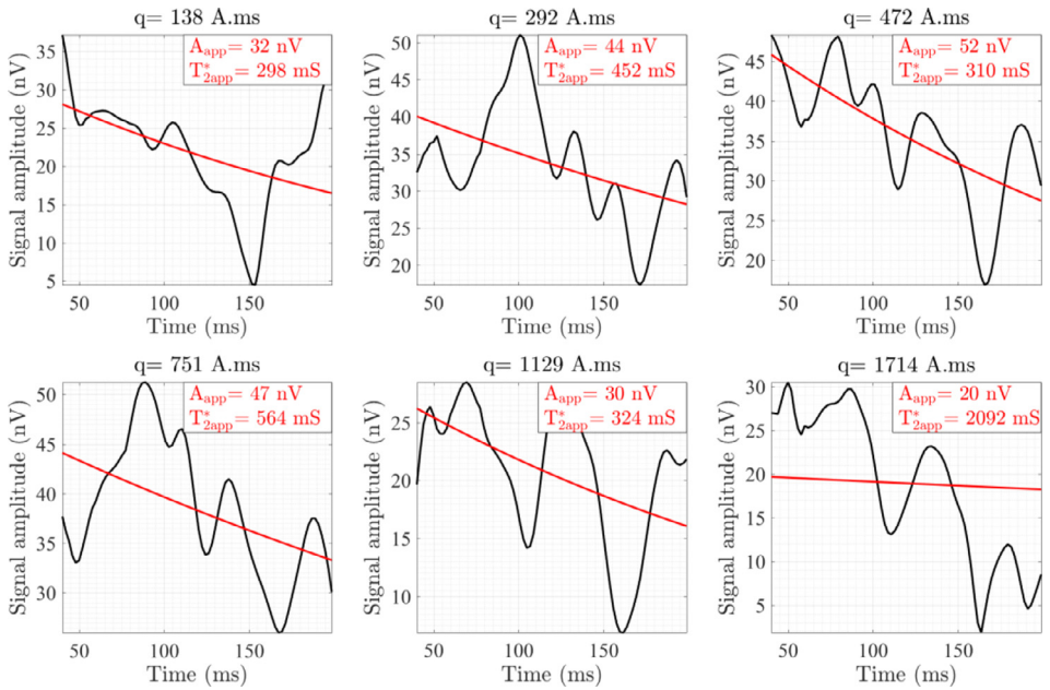
Fig. 16. Recorded signal at station 22.
