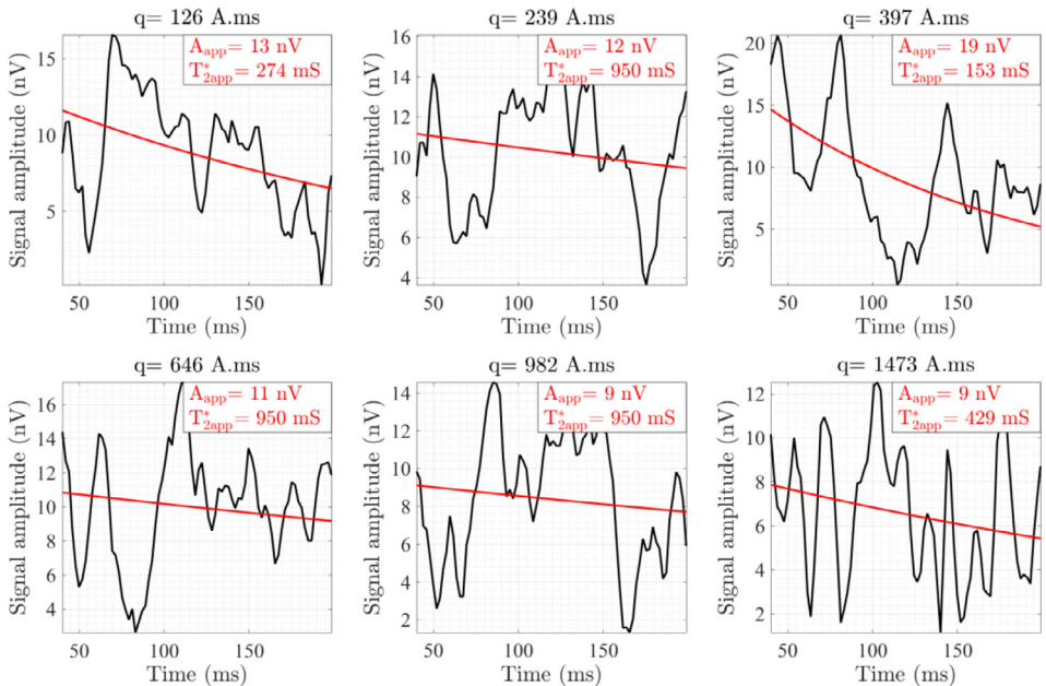
Fig. 12. Recorded signal at station 14.
