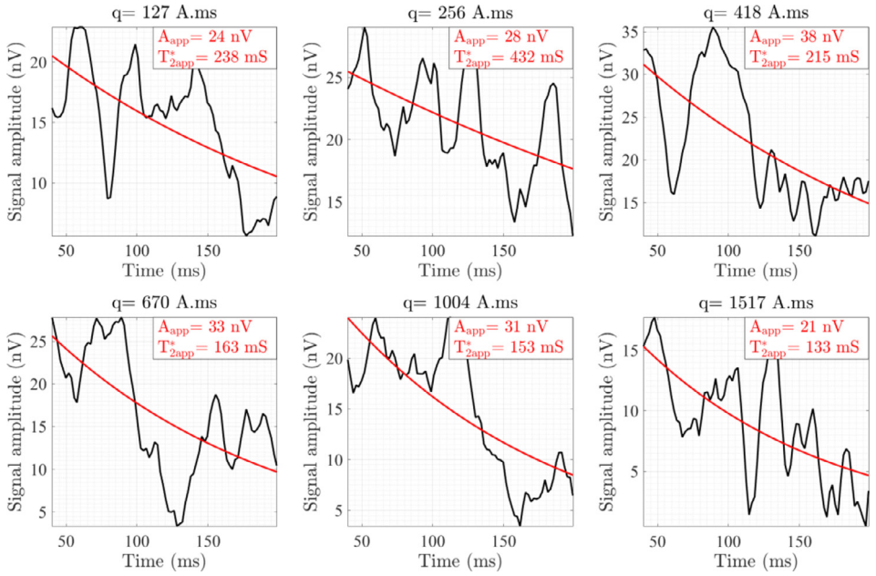
Fig. 7. Recorded signal at station 7.
