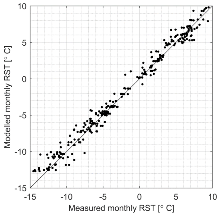
785 Figure 5: Mean modelled vs. measured monthly RST for all locations RW01 to RW08, comprising each entirely recorded month for the measurement periods stated in Table 1.
