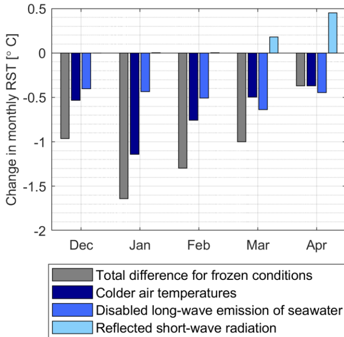
790 Figure 6: Temperature difference between the open fjord scenario (reference) and different model scenarios. “Colder air temperature”: as reference, but using colder air temperature as distance to the open water body is enlarged; “No seawater long-wave emission”: as reference but using air temperature instead of seawater temperature; “Reflected short-wave radiation”: as reference but assuming ice albedo for the surrounding terrain; “Total difference”: frozen bay scenario combining all three effects.
