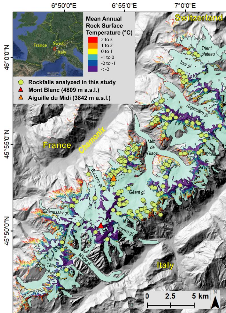
107 108 Figure 1. The Mont Blanc massif, the MARST distribution and the location of rockfalls analyzed in this study. 109
