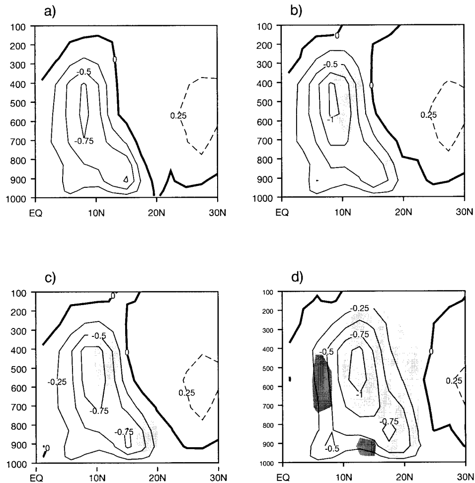
FIG. 12. Vertical velocity ( 10^{-3} \text{ hPa s}^{-1} ) plotted as a function of latitude and altitude, zonally averaged over Africa ( 10^{\circ}\text{W} – 30^{\circ}\text{E} ) for JJAS. (a) The simulated present-day climate, (b) the orbitally induced mid-Holocene climate (OF), (c) the mid-Holocene climate simulated in response to both orbital and SST forcing (OFSST), and (d) the mid-Holocene climate simulated in response to both orbital and vegetation forcing (OFGS). Negative values (i.e., ascending motion) are plotted using solid lines, and positive values (i.e., subsidence) using dashed lines. Isolines are every 0.25 \times 10^{-3} \text{ hPa s}^{-1} . Light shading corresponds to regions where the upward motion is increased; dark shading corresponds to regions where the upward motion is decreased.
