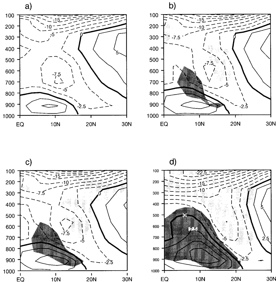
FIG. 13. Zonal wind ( \text{m s}^{-1} ) plotted as a function of latitude and altitude, zonally averaged over Africa ( 10^{\circ}\text{W} – 30^{\circ}\text{E} ) for JJAS. (a) The simulated present-day climate, (b) the orbitally induced mid-Holocene climate (OF), (c) the mid-Holocene climate simulated in response to both orbital and SST forcing (OFSST), and (d) the mid-Holocene climate simulated in response to both orbital and vegetation forcing (OFGS). Negative values (i.e., easterly wind) are dashed. Regions of increased easterly wind are lightly shaded while regions of decreased easterly wind are heavily shaded. Isolines are every 2.5 \text{ m s}^{-1} .
