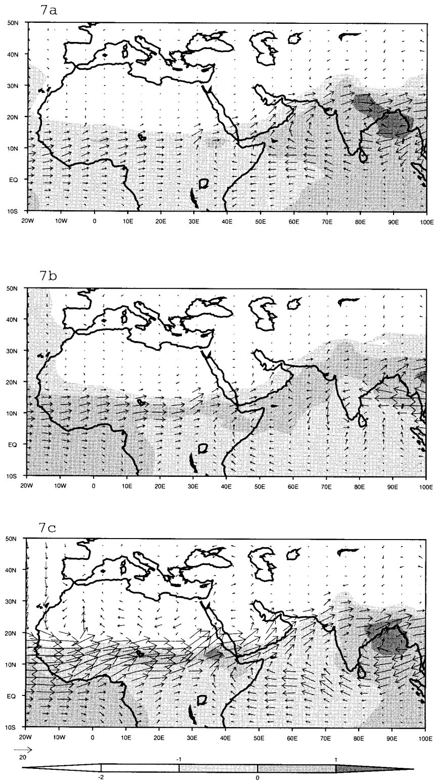
FIG. 7. Changes in the transport of latent heat ( 10^8 \text{ W m}^{-1} ) in the boundary layer in JJAS. Differences are between the simulated mid-Holocene climate and control. (a) The effect of orbital forcing alone (OF - Ctrl), (b) the combined effects of orbital forcing and SST changes (OFSST - Ctrl), and (c) the combined effects of orbital forcing and changes in the vegetation distribution (OFGS - Ctrl). Changes in SLP are shaded.
