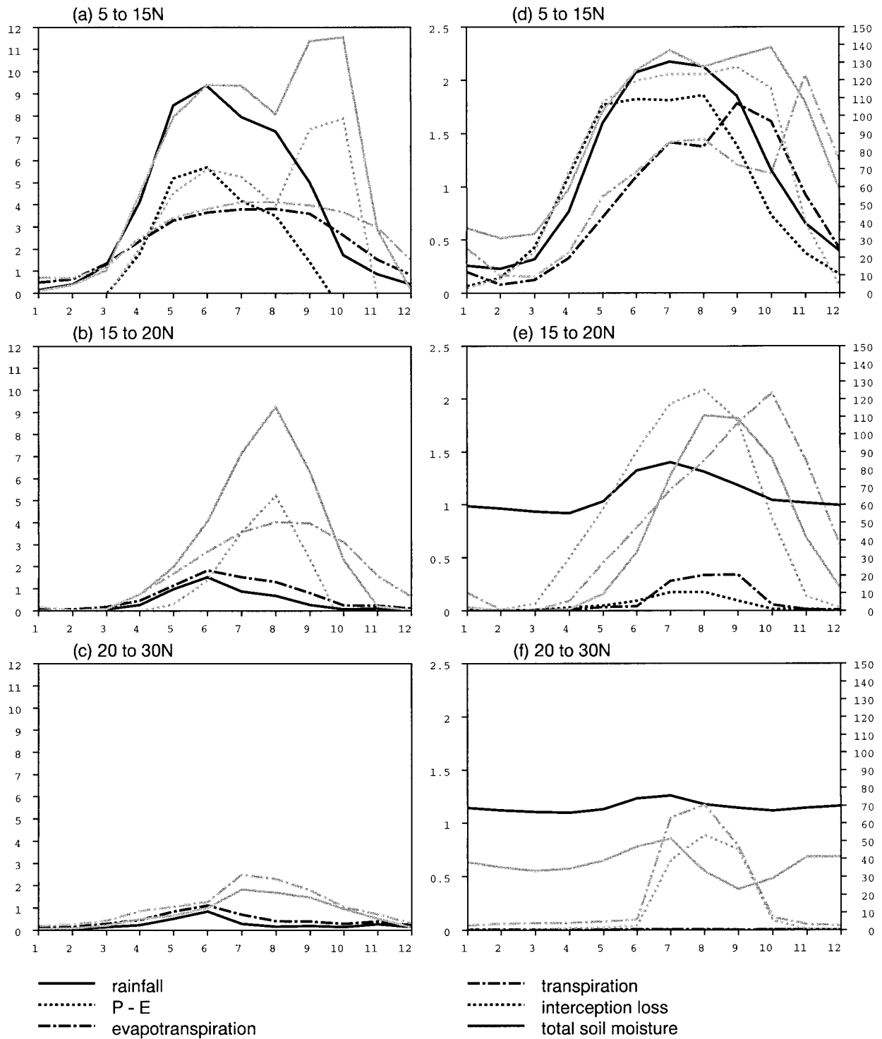
FIG. 10. Time evolution of mean quantities in northern Africa for Ctrl and OFGS. Averages are made longitudinally from 10°W to 30°E, and zonally from 5° to 15°N (a) and (d), 15° to 20°N (b) and (e), and 20° to 30°N (c) and (f). (left) The evolution of rainfall (plain lines), evapotranspiration (dashed-dotted lines), and difference between precipitation and evapotranspiration ( P - E ; dotted lines); (right) the evolution of total soil moisture in the root zone (plain lines), transpiration (dashed-dotted lines), and interception loss (dotted lines). The present-day simulation is represented using black lines, while OFGS is represented using gray lines.
