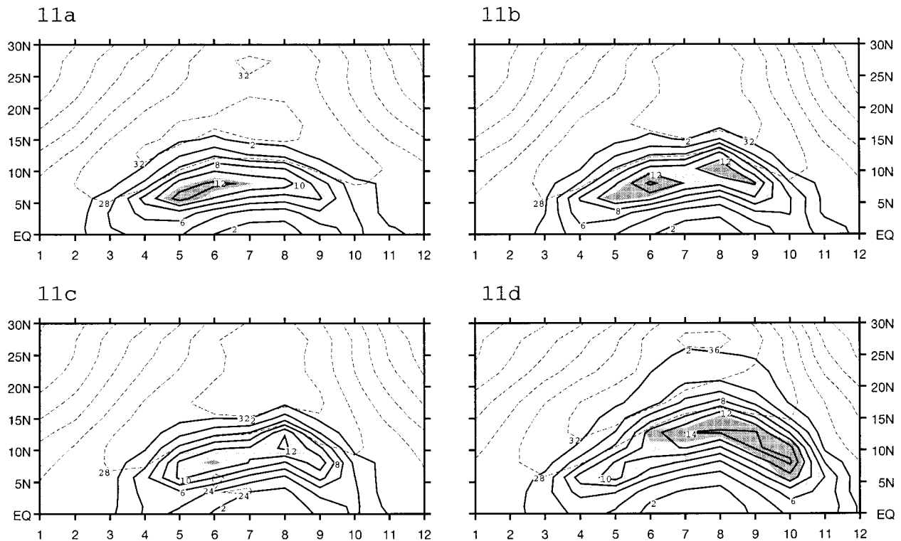
FIG. 11. Time evolution of precipitation ( \text{mm day}^{-1} , solid line) and surface air temperature ( ^{\circ}\text{C} , dashed line), zonally averaged over Africa ( 10^{\circ}\text{W} – 30^{\circ}\text{E} ) and plotted as a function of latitude. The shaded values represent the latitudes where, and the time when, the latent heat transport dominates the local recycling (i.e., P - E > evapotranspiration) in the rainfall term. (a) The simulated present-day climate, (b) the orbitally induced mid-Holocene climate (OF), (c) the mid-Holocene climate simulated in response to both orbital and SST forcing (OFSST), and (d) the mid-Holocene climate simulated in response to both orbital and vegetation forcing (OFGS). Isolines are every 2 \text{ mm day}^{-1} for precipitation and every 4^{\circ}\text{C} for temperature.
