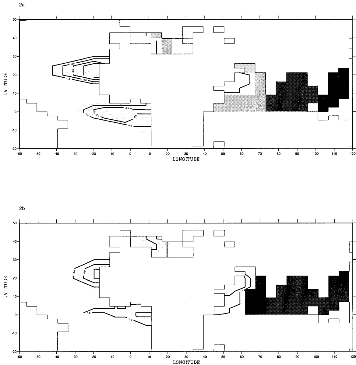
FIG. 2. Prescribed changes in SSTs ( ^{\circ}\text{C} ) for the mid-Holocene, for months of (a) Feb and (b) Aug. Isolines are -1^{\circ} , -2^{\circ} , -3^{\circ} , and -4^{\circ}\text{C} . Shading from the lightest to the darkest are for differences 1) lower than -0.5^{\circ}\text{C} , 2) from -0.5^{\circ} to 0^{\circ}\text{C} , 3) from 0^{\circ} to 0.5^{\circ}\text{C} , and 4) larger than 0.5^{\circ}\text{C} .
