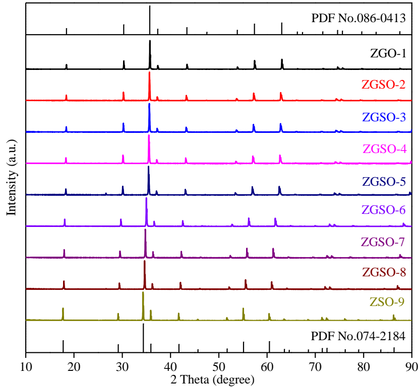
Figure 2. XRD patterns of complex spinel ZGSO, the standard data for \text{ZnGa}_2\text{O}_4 (PDF No.086-0413) and \text{Zn}_2\text{SnO}_4 (PDF No.074-2184).
