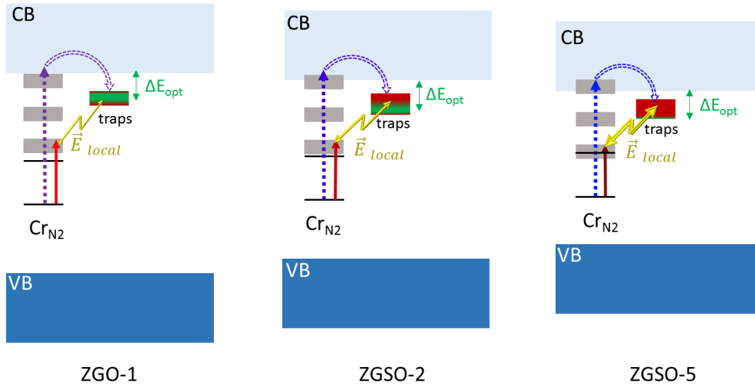
Figure 14: Schematic representation of the energy diagram evolution to model the evolution of the luminescence properties with the material composition. In this scheme, the trapping through the charge transfer from \text{Cr}^{3+} to the conduction band is represented by dotted arrows. The decreasing energy required for this process is schematized by the decreasing size and the color shift of the arrows from violet to blue. The trapping through the chromium bands is represented by the red solid arrows and their required energies are schematized by their size and tint. The local electric field that triggers the charging through chromium bands is represented by the yellow “lighting” arrows. Its efficiency is schematized by the arrows thickness. The red part of the traps represents traps that are not involved in the persistent luminescence process (traps that are too deep or too shallow for instance) whereas the green part represents the “useful” part when bioimaging applications are envisioned.
