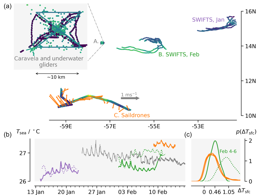
Figure 17. Near-surface temperature ( T_{\text{sea}} ) from drifters and gliders in the three EUREC 4 A study regions. Panel (a) shows the tracks of the instruments colored by T_{\text{sea}} . The magnification (upper left) expands the domain of the Caravela (and underwater glider) measurements in Region A (near 57° W). January and February SWIFT buoy ( T_{\text{sea}} at -0.3 m) deployments in Region B. Saildrone ( T_{\text{sea}} at -0.5 m) measurements across an eddy near 11° N, with anti-cyclonic currents (at -5 m) shown by vectors, in Region C. Panel (b) shows time series of T_{\text{sea}} measurements by the different instruments. Probability density, p , of air–sea temperature differences measured by two SWIFT buoys between 04:00 UTC 4 February and 14:00 UTC 6 February (c).
