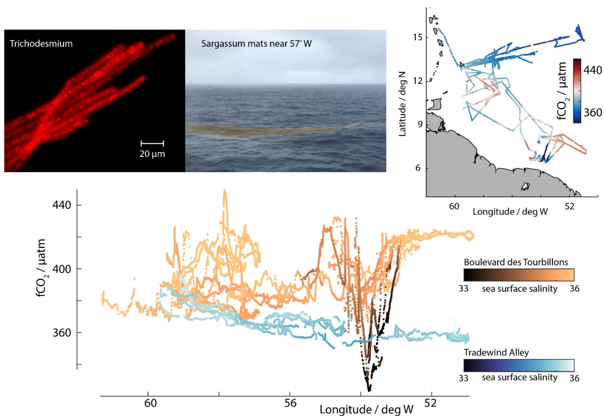
Figure 18. Measurements of CO 2 fugacity ( f\text{CO}_2 ) from the different surface vessels shown versus longitude (lower panel). The presentation contrasts strong variability in f\text{CO}_2 in association with eddies and salinity variations along Boulevard des Tourbillons (oranges in lower panel, track in upper right) versus in the Tradewind Alley (blues). Microscopic/epifluorescence image of several filaments of Trichodesmium , an N 2 -fixing cyanobacterium that is found in the region (upper left), and mats of seaweed ( Sargassum , photo W. Mohr, upper center) which were frequently observed and difficult to navigate from some of the uncrewed surface vehicles.
