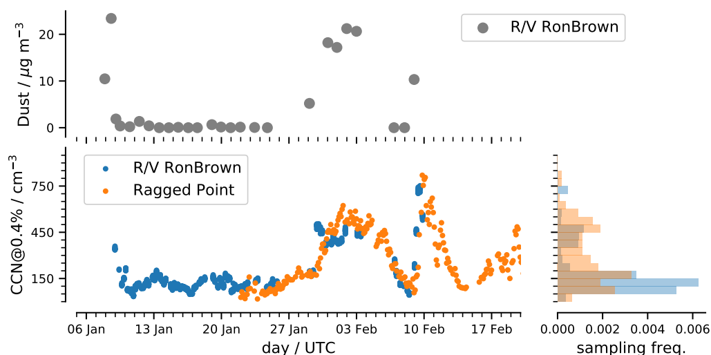
Figure 12. Aerosol characteristics in the Tradewind Alley over the period of measurements. Dust mass density from the R/V Ron Brown (upper left), which was mostly east of 55^\circ\text{W} . Normalized histogram showing the relative frequency of occurrence of different CCN concentration levels (lower right). Note that the periods of observation at the two locations are only partly overlapping.
