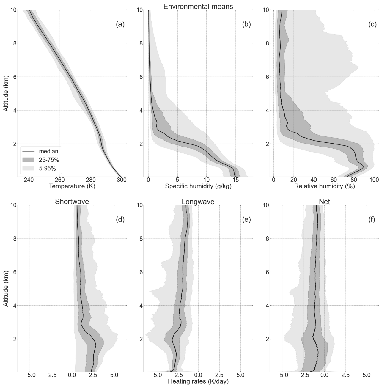
Figure 2. Top: Temperature (a), specific humidity (b) and relative humidity (c) (with respect to ice for T < 0^{\circ}\text{C} ) from EUREC 4 A dropsonde and radiosonde data. Bottom: Shortwave (d), longwave (e) and net (f) heating rates calculated from EUREC 4 A dropsonde and radiosonde data using the radiative transfer code RRTMGP. The center traces are the median profiles, and the medium and light grey shadings indicate the 25–75% and 5–95% intervals, respectively. For the shortwave, the median and the interquartile range are calculated using daytime values only.
