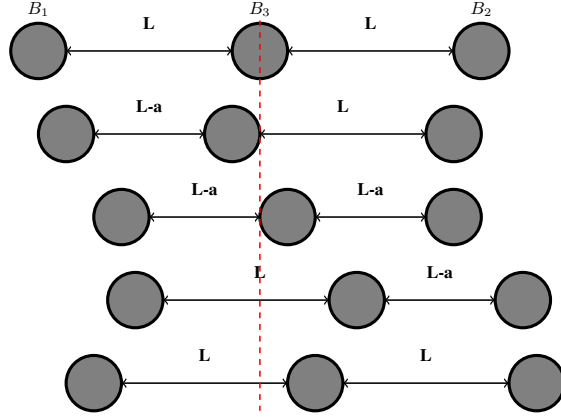
Figure 1: Representation of the three-sphere swimmer and its swimming gait. The gait is composed of four strokes in which one of the arms is alternatively shrunken or elongated. The alternation guarantees the non-reciprocity of the motion.
