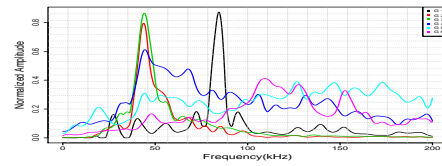
(b) Superposition of the normalized mean spectra for the six clusters.
