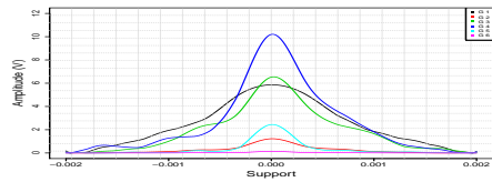
(a) Superposition of the mean envelopes for the six clusters.
