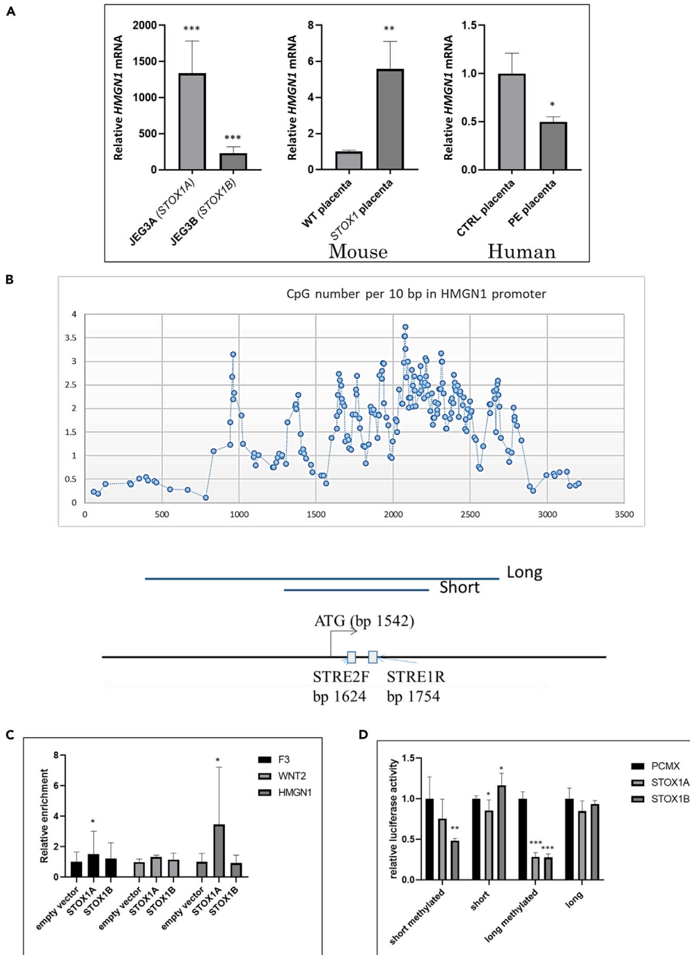
Figure 7. Analysis of HMGN1 Expression in Cells and Placentas
