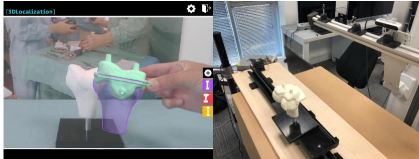
Figure 1: The prototype tracking application showing planned femur and PSI hologram, and the test bench.
