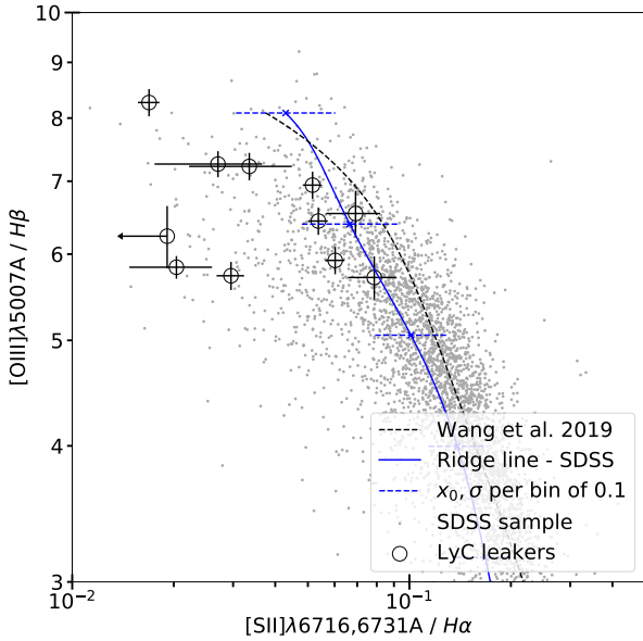
Fig. 1. O3H\beta – S2H\alpha diagram of the LyC leakers (open circles) and comparison sample with metallicities 12 + \log(O/H) = 7.6 – 8.2 (gray dots). The plain blue line shows the ridge line of our SDSS sample, and the black dashed line is the ridge line from Wang et al. (2019) extrapolated to high [O\text{ III}]/H\beta values. Many leakers, especially the strongest ones, show a deficiency in [S\text{ II}] with respect to this latter ridge line.
