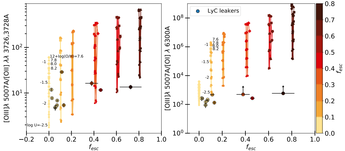
Fig. 6. Observed and predicted [O\text{ III}]/[O\text{ II}] (left) and [O\text{ III}]/[O\text{ I}] (right) line ratios as a function of the LyC escape fraction, comparing the observed LyC emitters and the one-zone photoionization models with \log(U) \gtrsim -2.5 . We note the very high range of the predicted [O\text{ III}]/[O\text{ I}] ratio.
