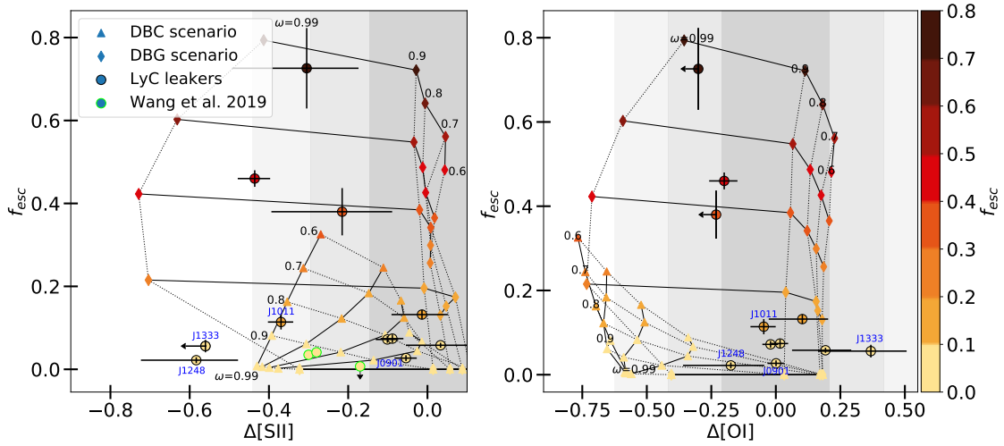
Fig. 11. LyC escape fraction as a function of the deficiency \Delta[\text{S II}] (left) and \Delta[\text{O I}] (right). The gray-shaded areas represent dispersion of the SDSS comparison sample at 1, 2, and 3 \sigma . The three strongest leakers (J1256+4509, J1154+2443 and J1243+4646, in increasing order of f_{\text{esc}} ) are represented by orange to brown circles in the upper part of the plots. The other galaxies that are discussed in Sect. 4.4 are labeled in blue.
