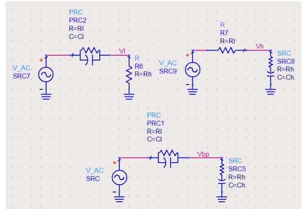
FIGURE 11. Design schematic of the simulated LP, HP and LP-HP NGD circuit.
