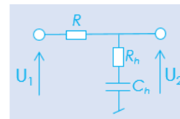
FIGURE 5. Elementary HP passive cell [33].
