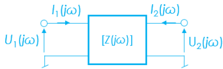
FIGURE 1. Two-port black box system represented by its impedance matrix.
