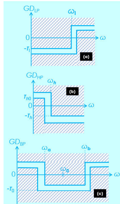
FIGURE 2. (a) LP, (b) HP, and (c) BP NGD ideal responses.
