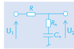
FIGURE 5. Elementary HP passive cell [33].
