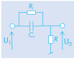
FIGURE 4. Elementary LP NGD passive cell [33].
