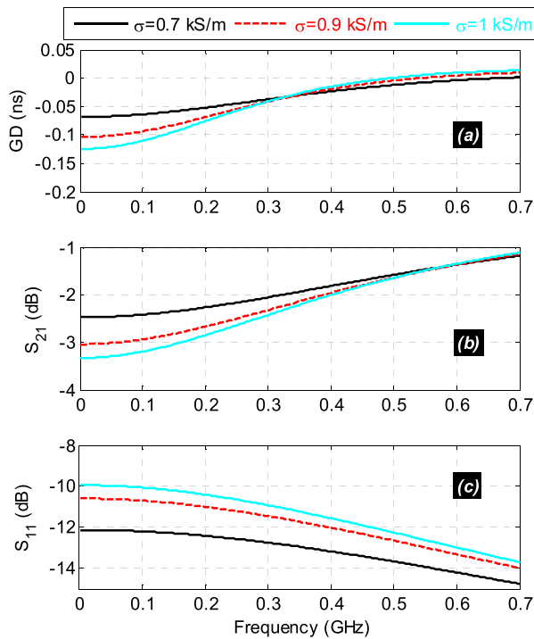
FIGURE 9. Calculated frequency responses: (a) GD, (b) transmission and (c) reflection coefficients of NGD via structure for conductivities \sigma = \{0.7 \text{ kS/m}, 0.9 \text{ kS/m}, 1 \text{ kS/m}\} .
