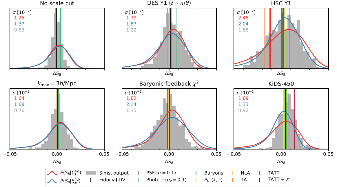
Figure 10. Distribution of differential biases \Delta\hat{S}_8 \equiv \hat{S}_8|_{\xi_{\pm}} - \hat{S}_8|_{C_\ell} between real space and harmonic space analyses. The histograms show the posterior mean difference derived from simulations. They are compared to individual posteriors, P(S_8|X) with X = C_\ell, \xi_{\pm} , derived from fiducial data vectors and shifted with respect to their own mean S_8 . Each panel corresponds to a different scale cut used in this analysis, as indicated above. The standard deviations (multiplied by 100) of the C_\ell posterior (red), \xi_{\pm} posterior (blue), and \Delta\hat{S}_8 histograms (grey) are reported in the upper left of each panel. Vertical lines indicate the differential biases computed for data vectors contaminated with unmodelled systematics.
